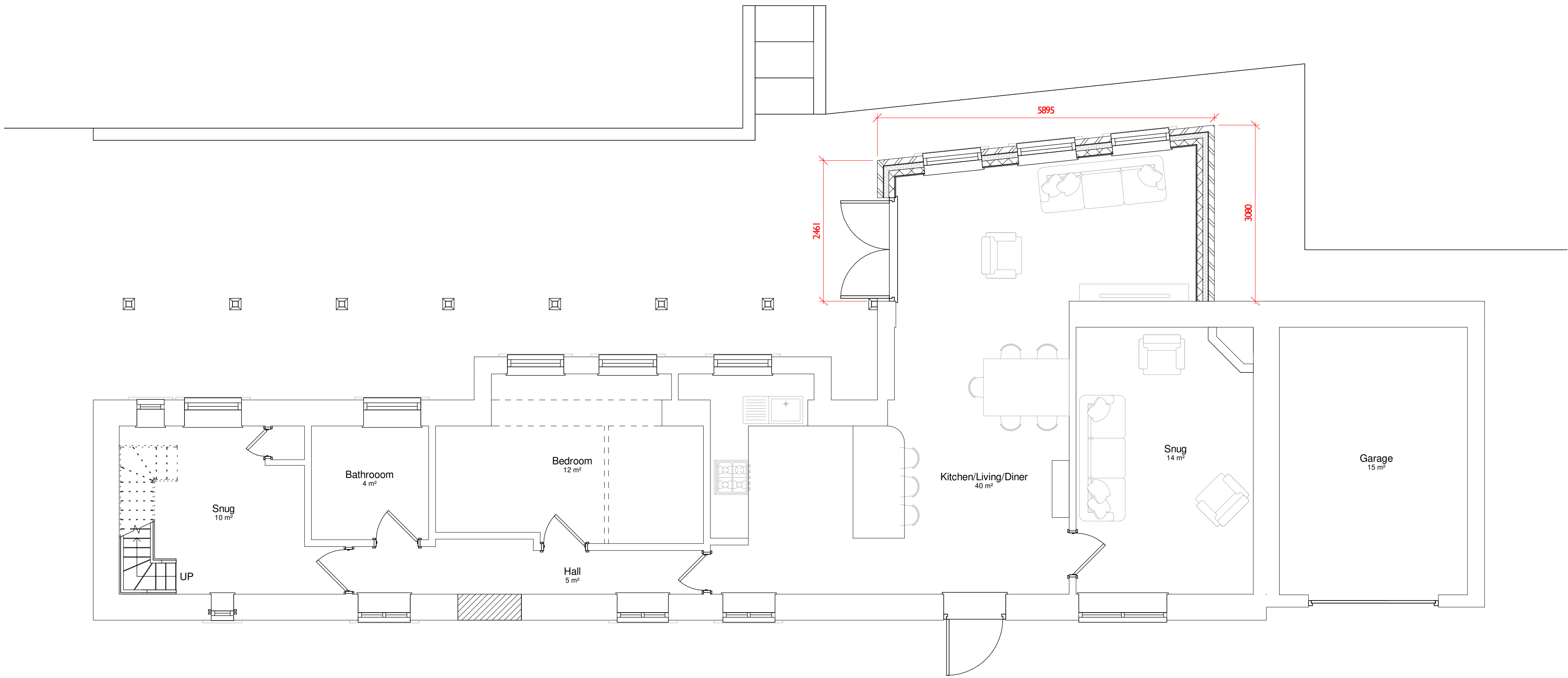
1 | Proposed_Level 00 1 : 50
