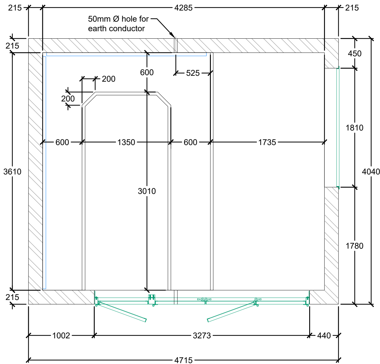
Substation - Typical Setting Out Dimensions N.T.S @ A1
