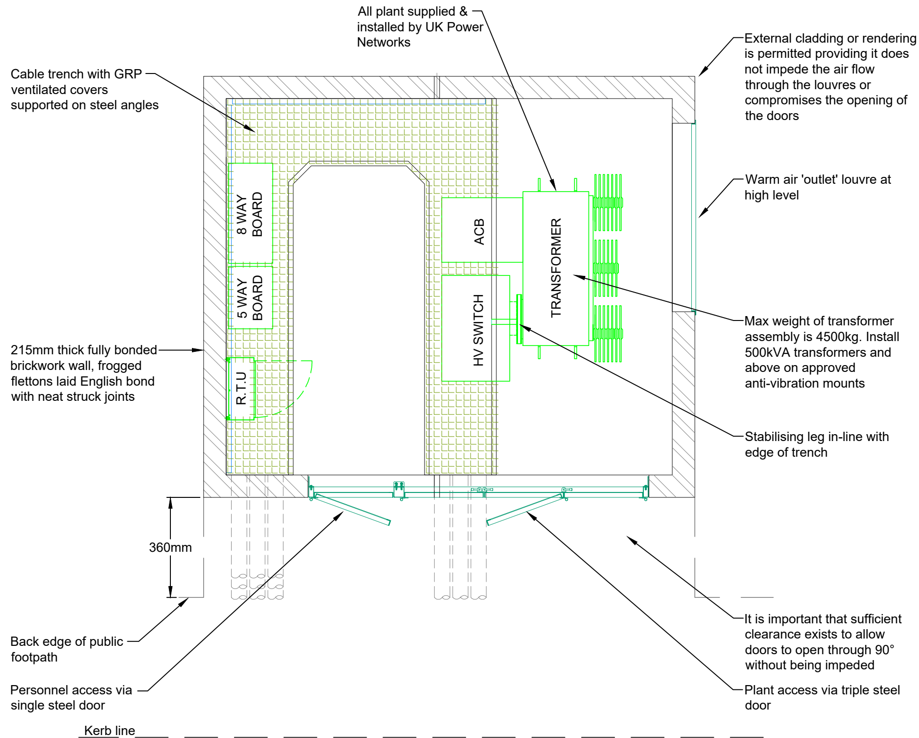
Typical Layout For A UKPN Substation N.T.S @ A1
