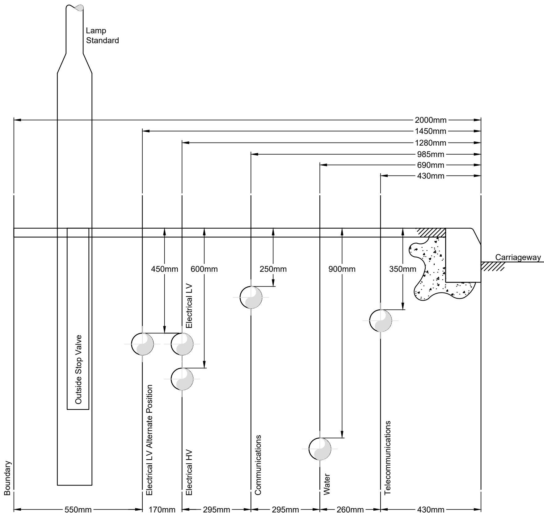
Typical Buried Service Detail 1 N.T.S @ A1
