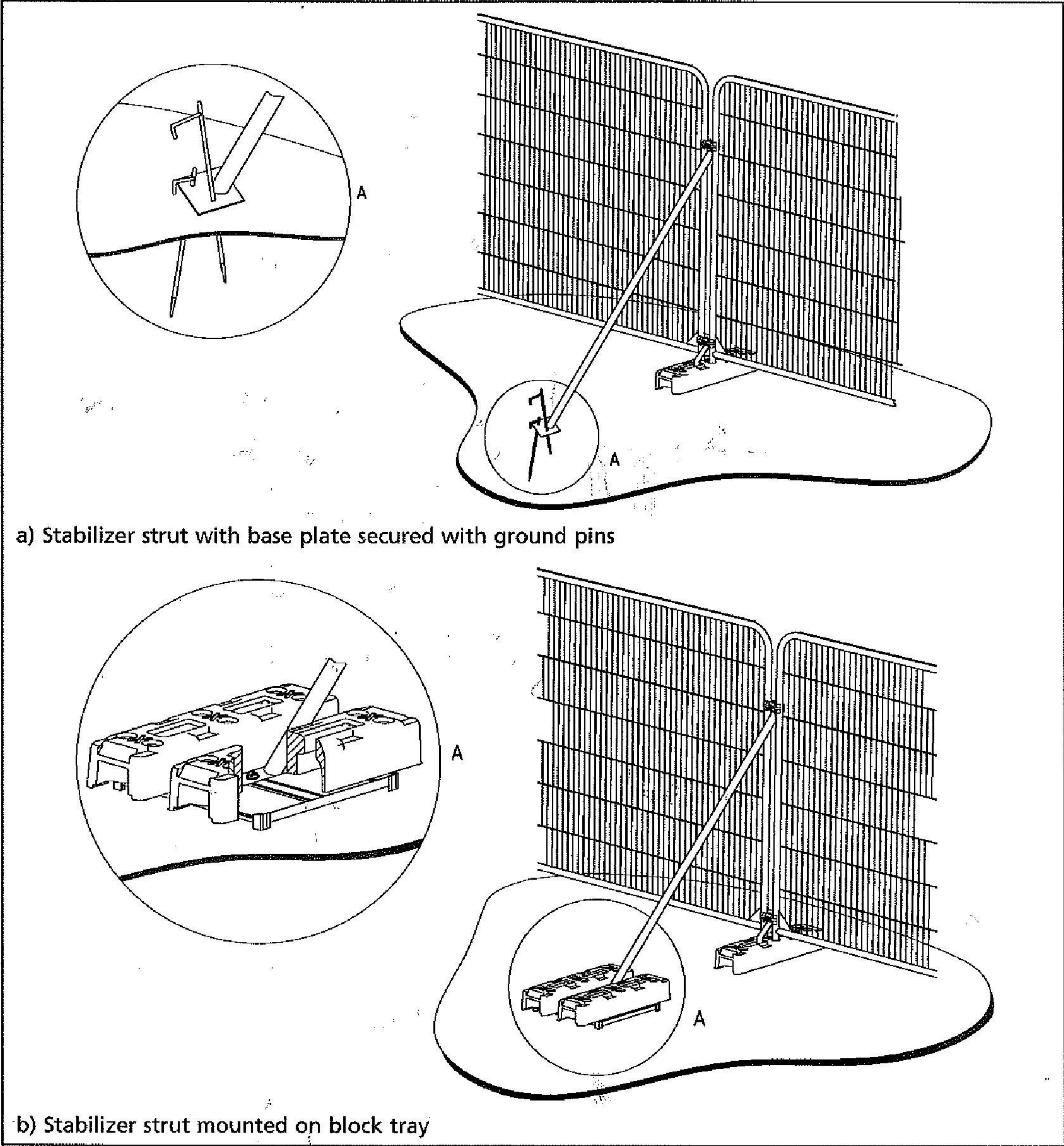
Figure 3 Examples of above-ground stabilizing systems
