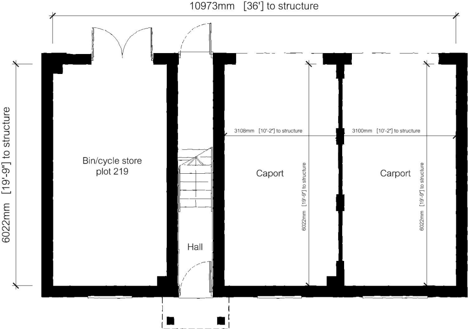
HT-SA Plot 219 Ground Floor Plan
