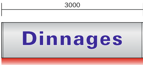
Sign 'C' Scale 1:50 APPROX Size - 3,000mm x 750mm - Plus silver endcaps Description - Rolled fascia panel with backed up 'DEALER' graphics with white keyline Materials - Aluminium (Fascia) Acrylic (Text) Illumination - Internally illuminated Height from ground level: 2625mm
