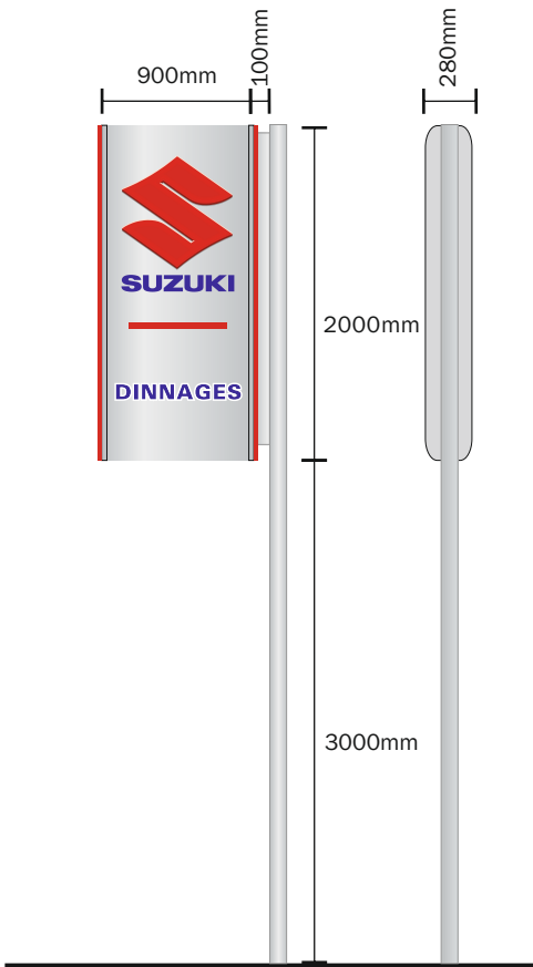
Sign 'A' Scale 1:50 Post Sign Rolled aluminium panels with silver endcaps. Fret cut with pushed through acrylic letters and standard moulded "S" Internally illuminated. Fitted onto existing steel post finished corporate grey. Cap height for 'Z' of SUZUKI = 98mm Cap height for 'D' of 'DINNAGES' = 92mm Logo height = 666mm
