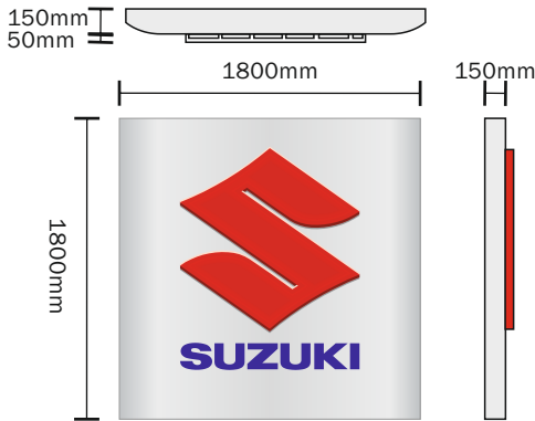
Sign 'B' Scale 1:50 Wall mounted sign Rolled and folded aluminium panel with moulded 'S' logo and text Size: 1800mm x 1800mm Cap height for 'Z' of SUZUKI = 160mm Logo height = 1050mm Illumination : Illuminated Height from ground level: 3675mm
