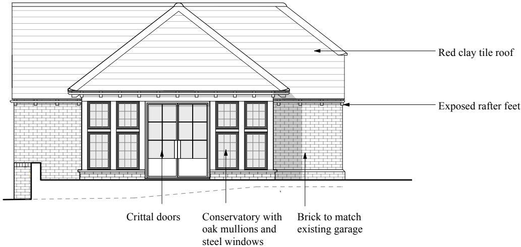
East Elevation
