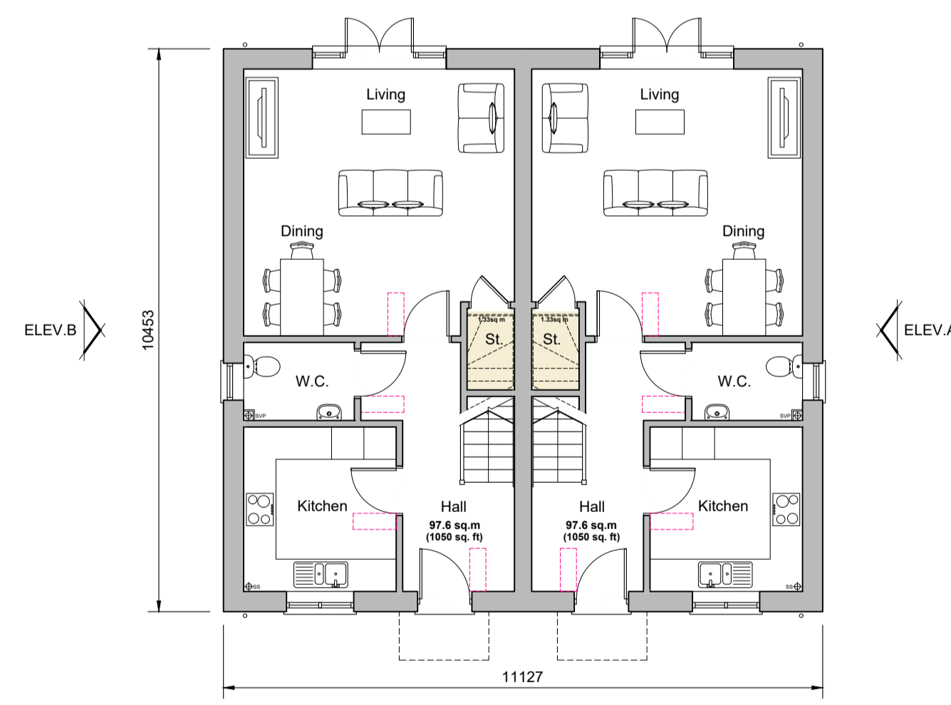
Ground Floor Plan Plots 29-30
