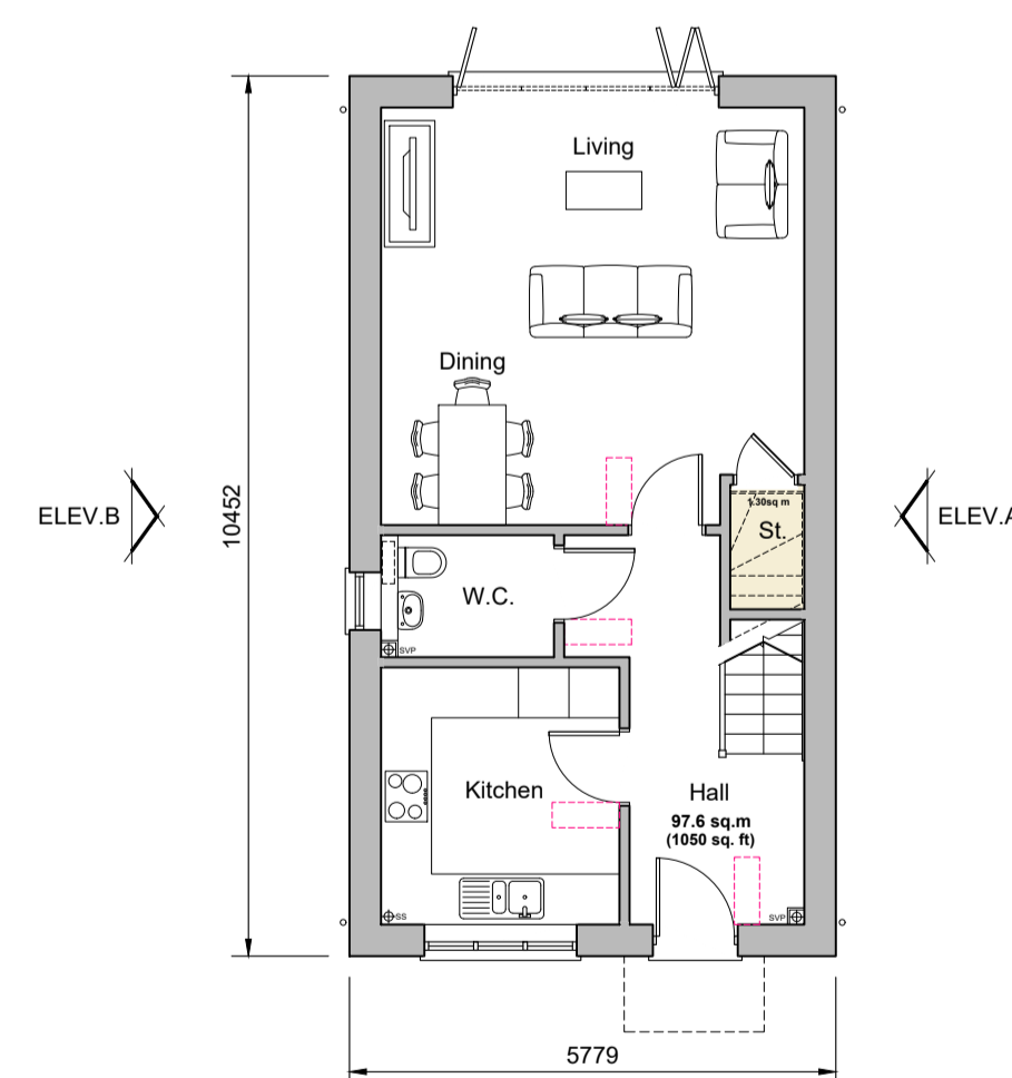
Ground Floor Plan Plot 8
