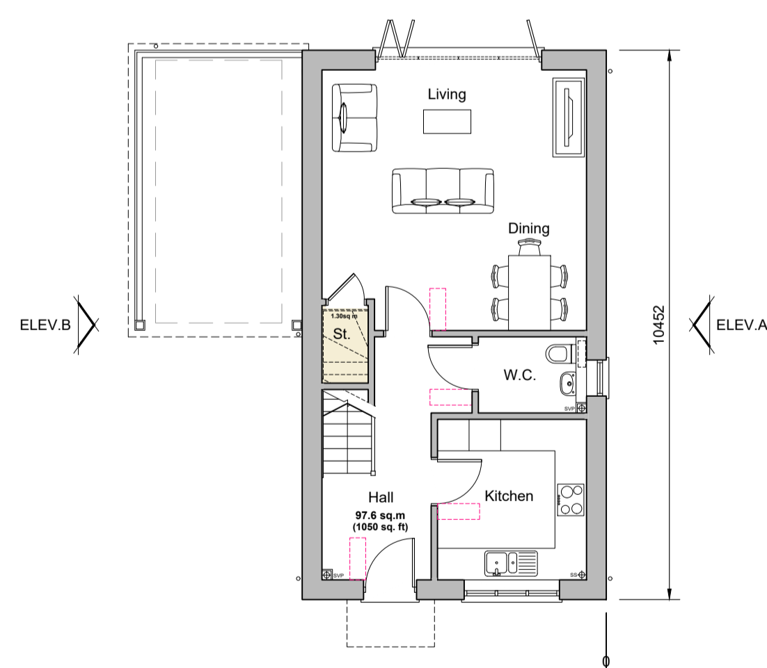
Ground Floor Plan Plot 15
