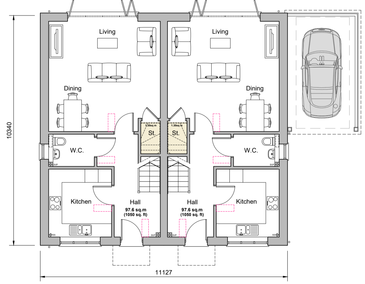
Ground Floor Plan Plots 13-14
