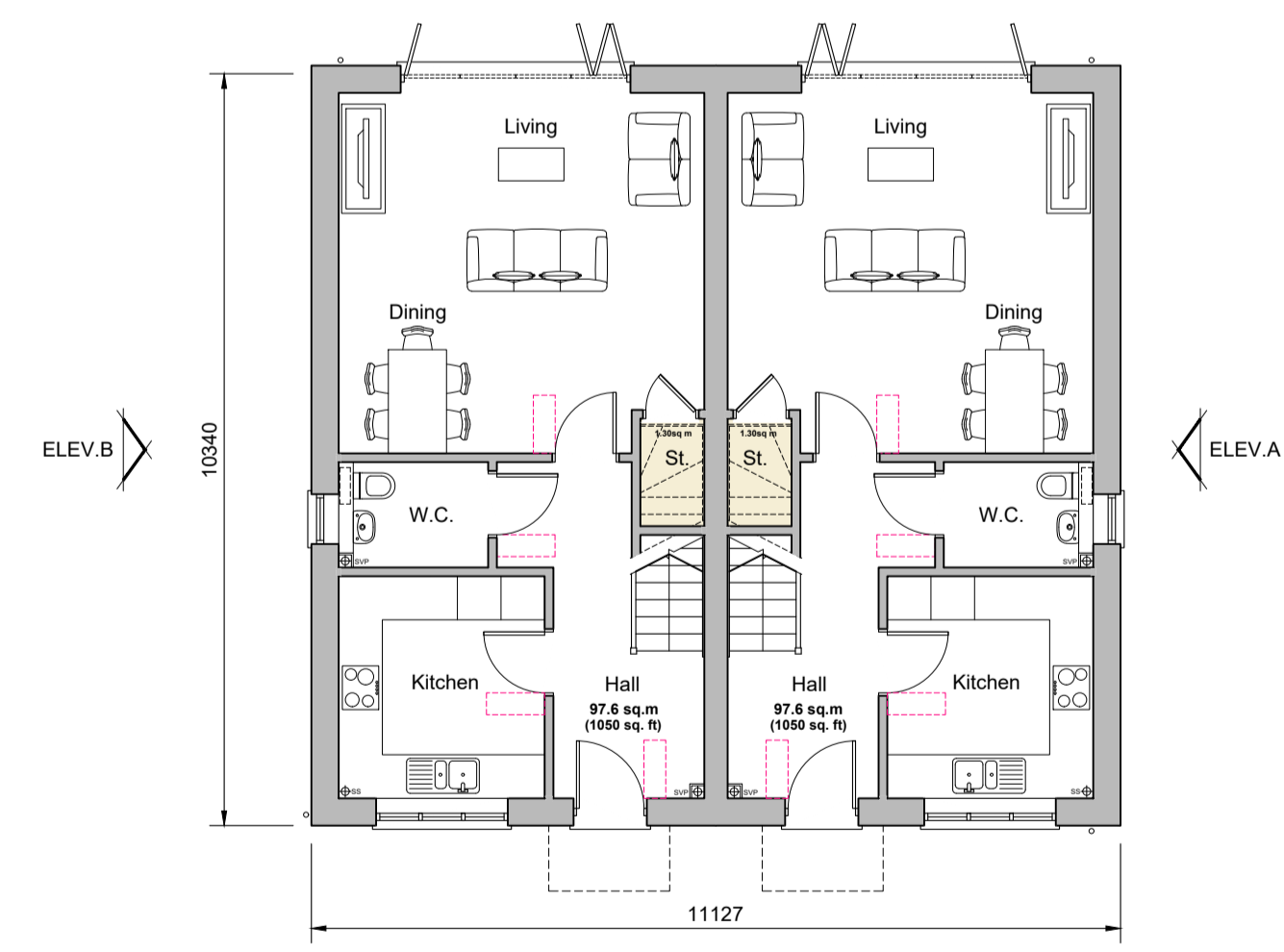
Ground Floor Plan Plots 19-20
