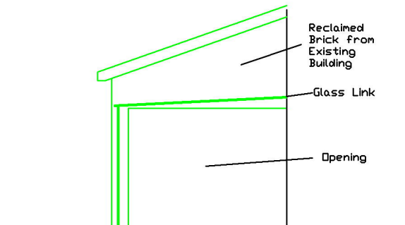
ELEVATION FROM WEST
