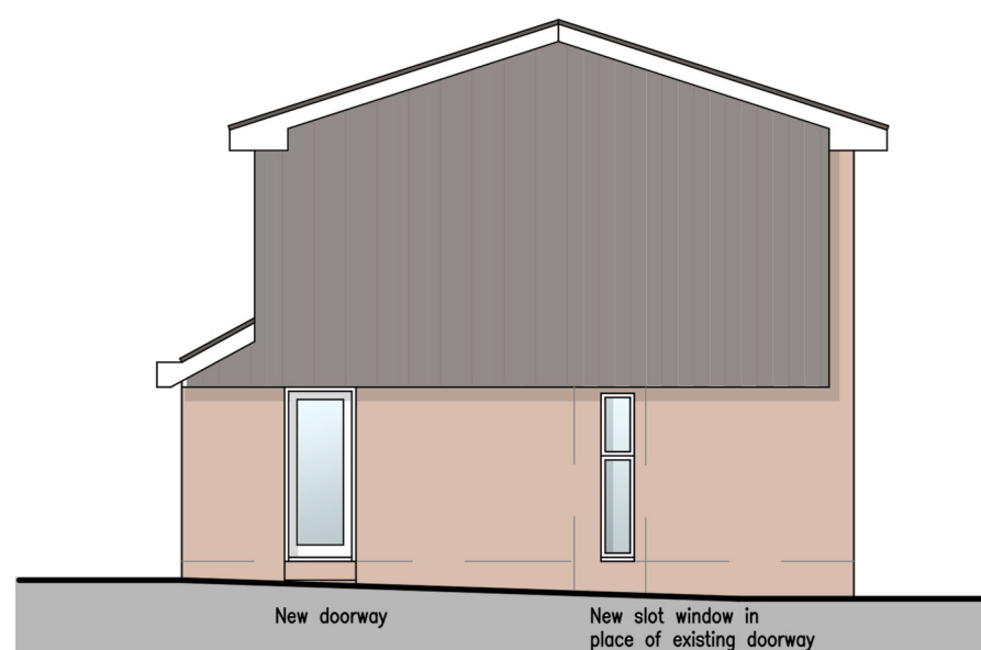
side elevation (ne) 1:100
