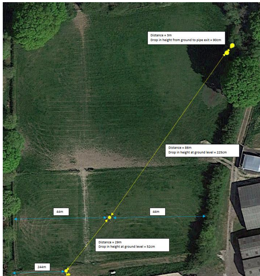
Figure 6: Extract of Existing Drainage Sketch Received from Applicant (2021)
