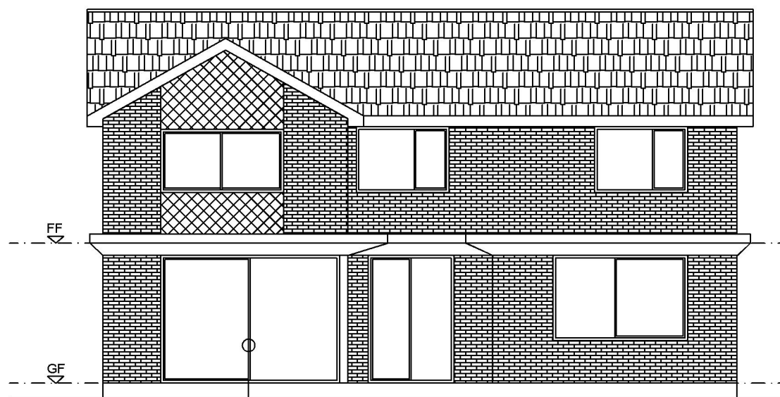
REAR ELEVATION
