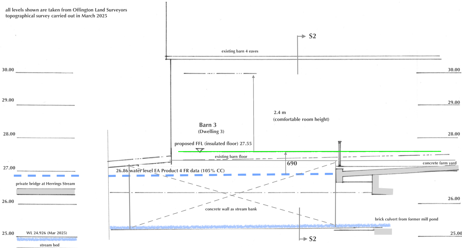
section at bridge
