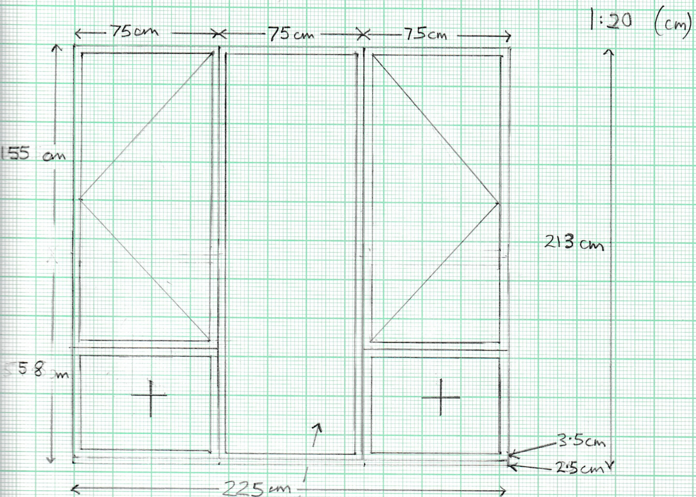
SOUTH BEDROOM WINDOW - PROPOSED ELEVATION
