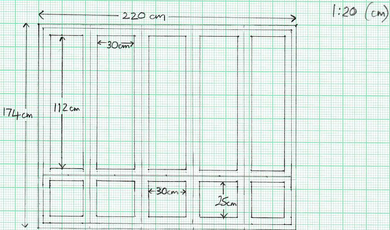
SOUTH BEDROOM WINDOW - EXISTING ELEVATION
