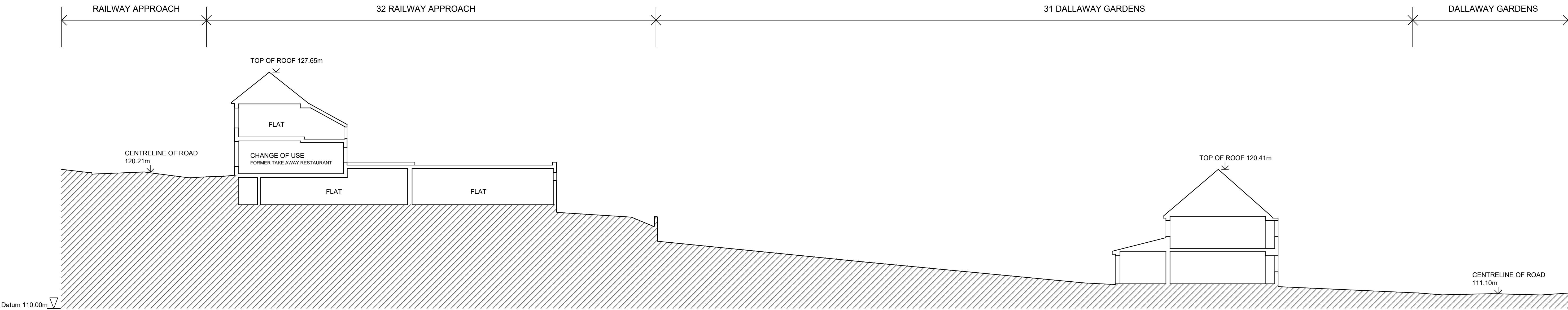
LONG SECTION TO DALLAWAY GARDENS
