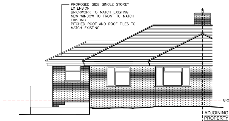
A) Proposed Front Elevation
