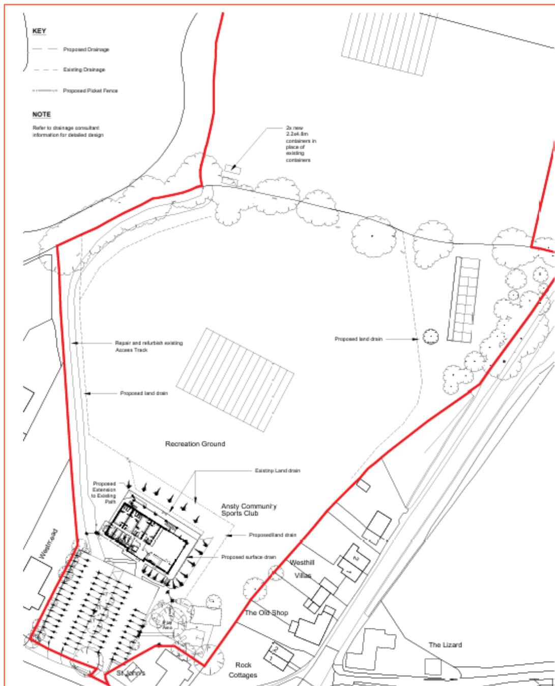
Figure 3: Proposed groundworks plan (Source: Applicant)
