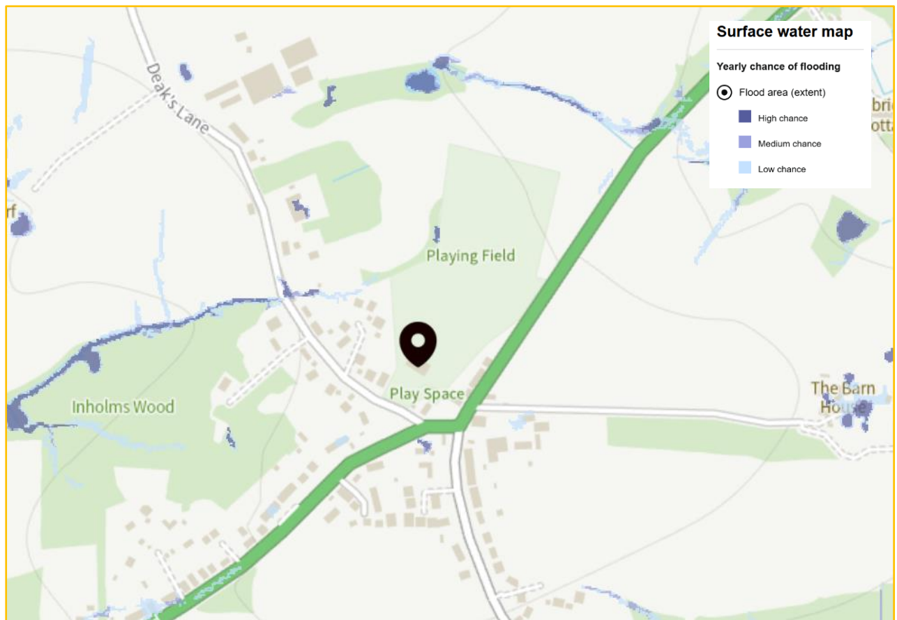
Figure 6: Extract from EA Risk of Flooding from Surface Water mapping – present day (Source: EA)
