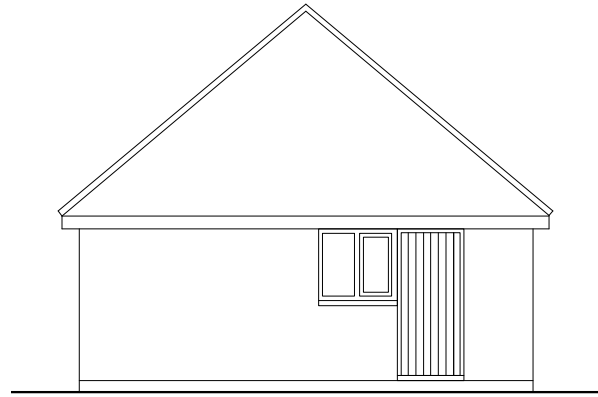
0 Consented side elevation B Scale: 1:100
