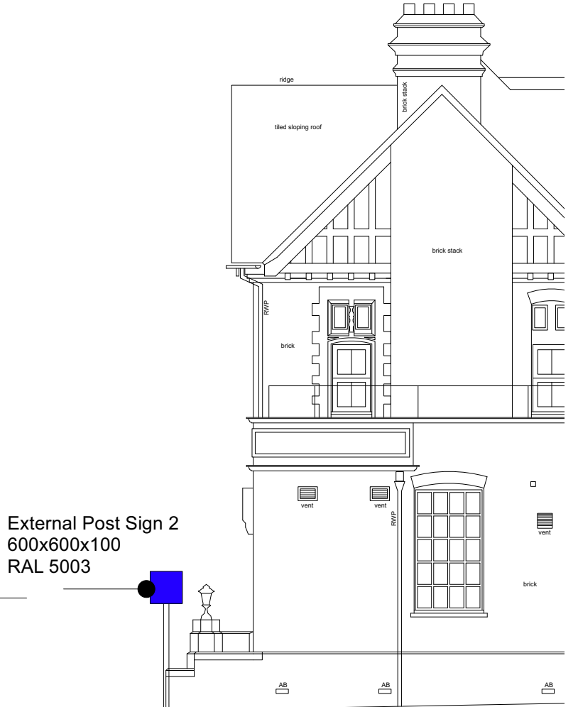
Elevation to Car Park Entrance [Part] South East 1:100
