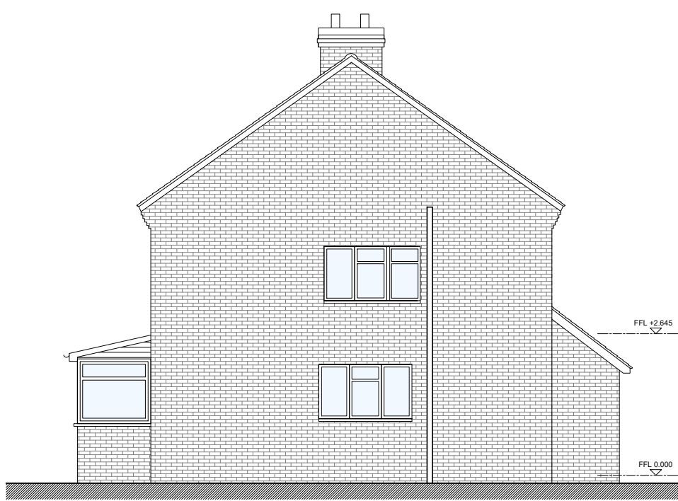
West Elevation (Side) 1:100
