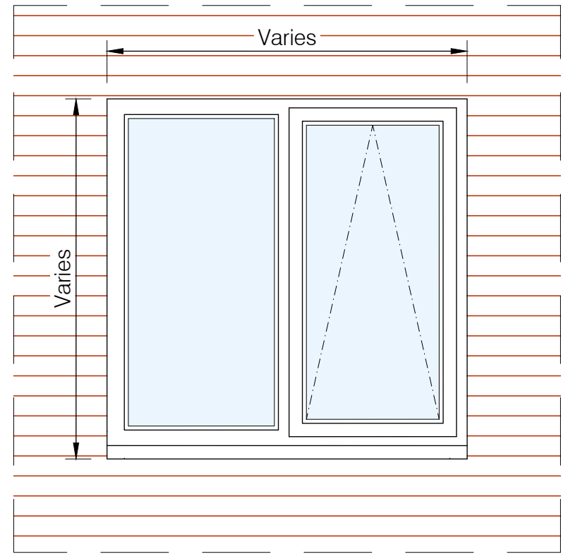
Window Elevation - Brick - Scale @ 1:20
