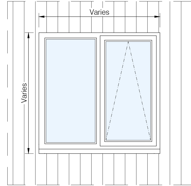
Window Elevation - Vertical Cladding - Scale @ 1:20
