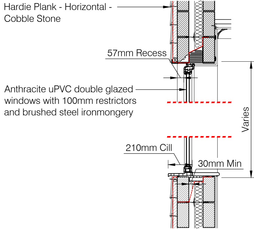
Window Detail - Horizontal Cladding - Scale @ 1:20
