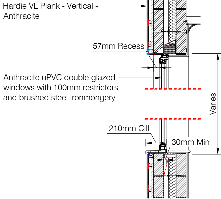
Window Detail - Vertical Cladding - Scale @ 1:20
