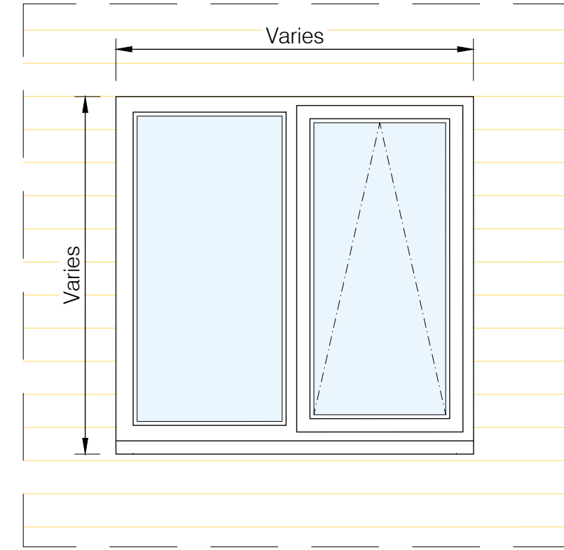
Window Elevation - Horizontal Cladding - Scale @ 1:20
