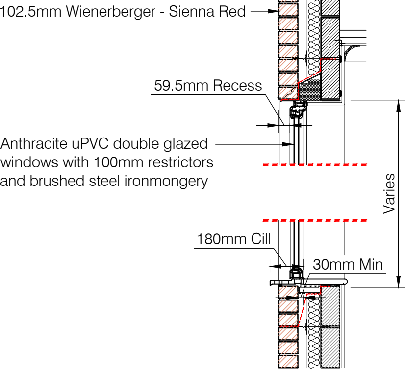
Window Detail - Brick - Scale @ 1:20
