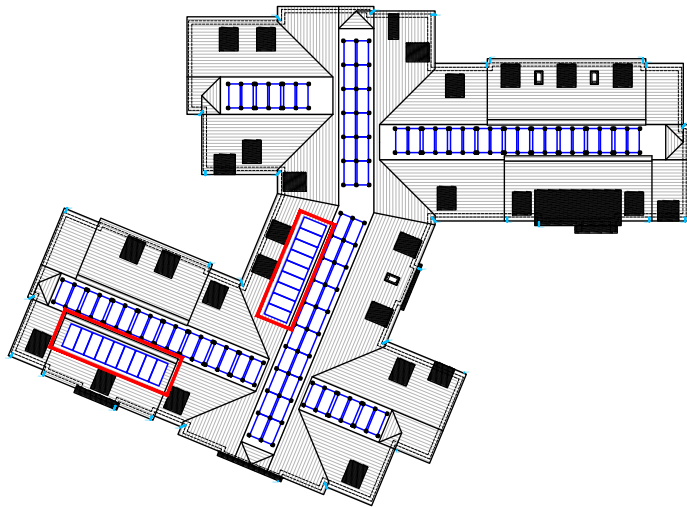
Location of Inset PV Panels - Scale @ 1:750
