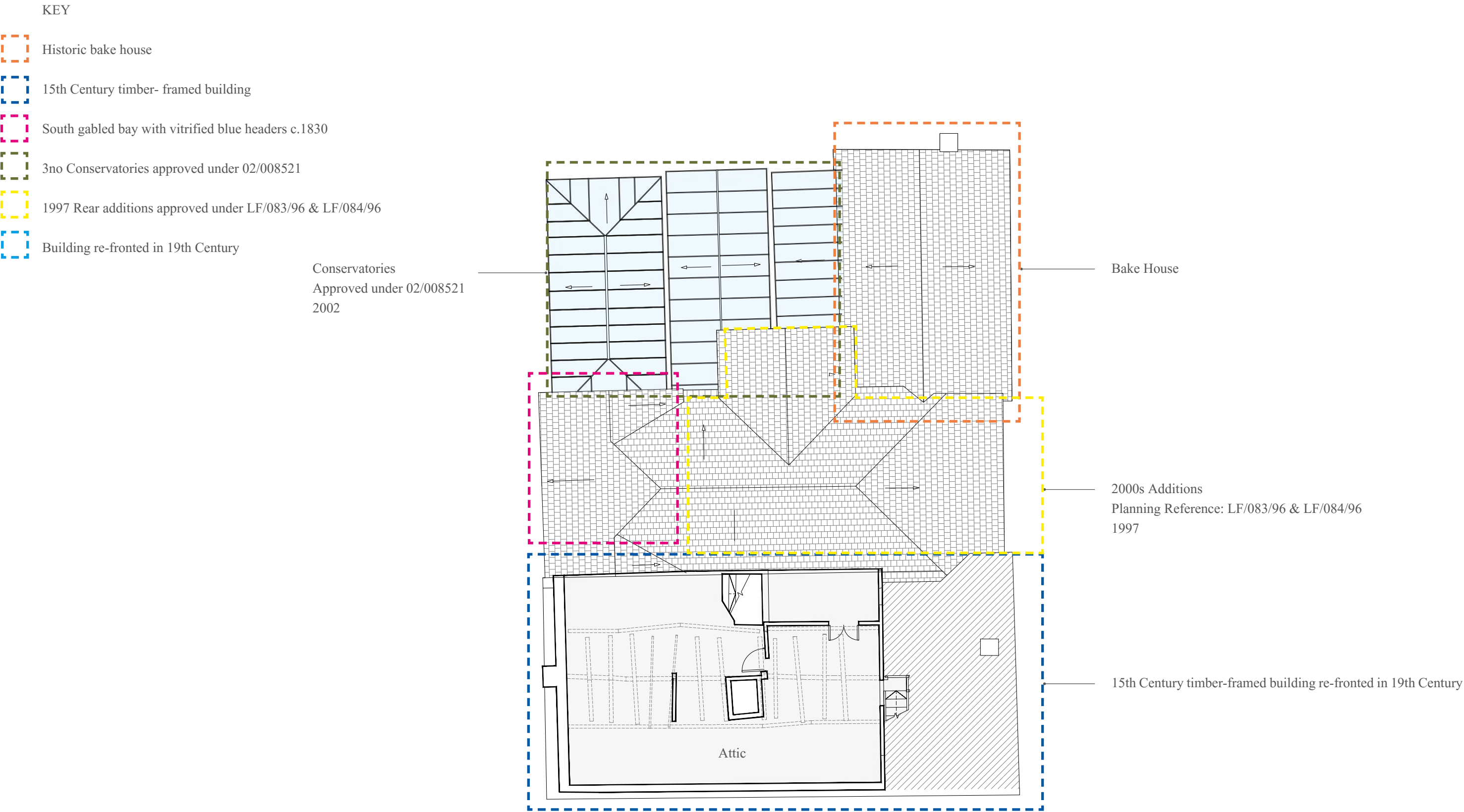
PRE-CONSTRUCTION - SECOND FLOOR PLAN. 1:100@A3
