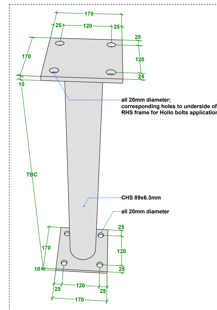
Pergola (East Elevation) - Steelwork Support Posts
