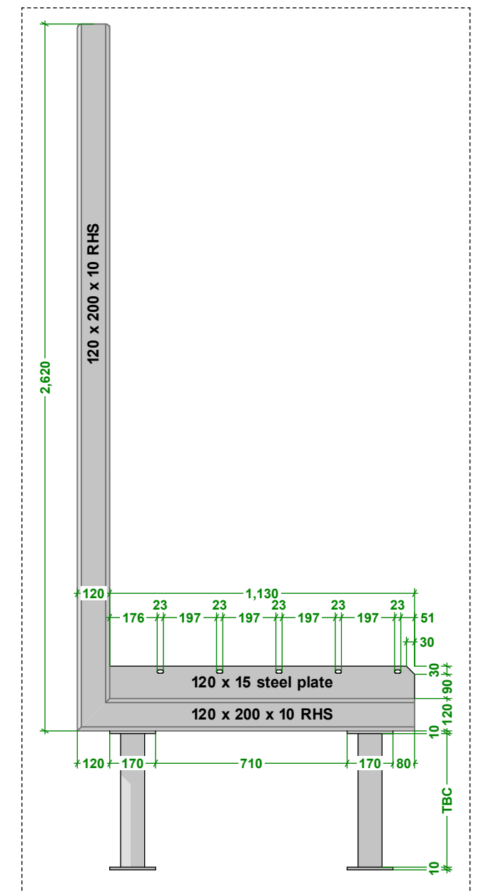
Pergola (East Elevation) - Steelwork Side View - Identical
