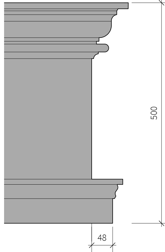
Proposed Cornice Details 1:5
