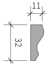
Proposed Decorative Arches Moulding Surround 1:2
