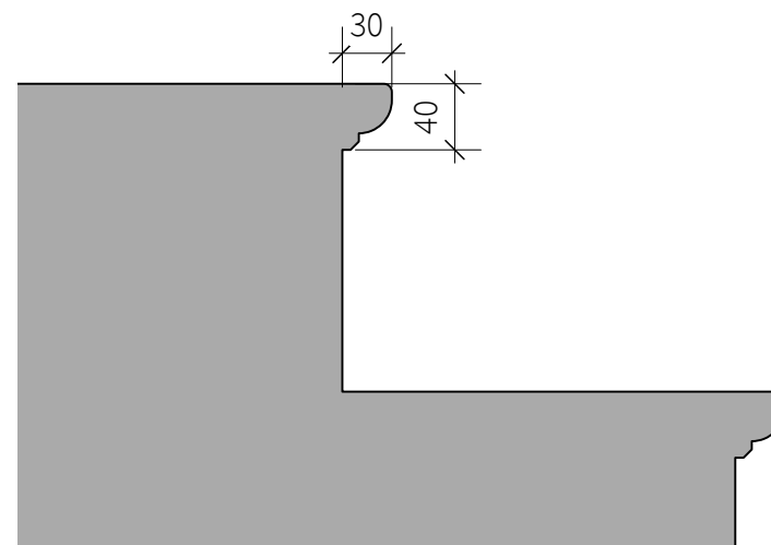
Proposed Stair Detail Oversail 1:10
