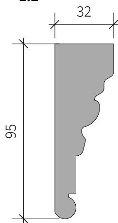
Proposed Skirting and Plinth Details 1:2
