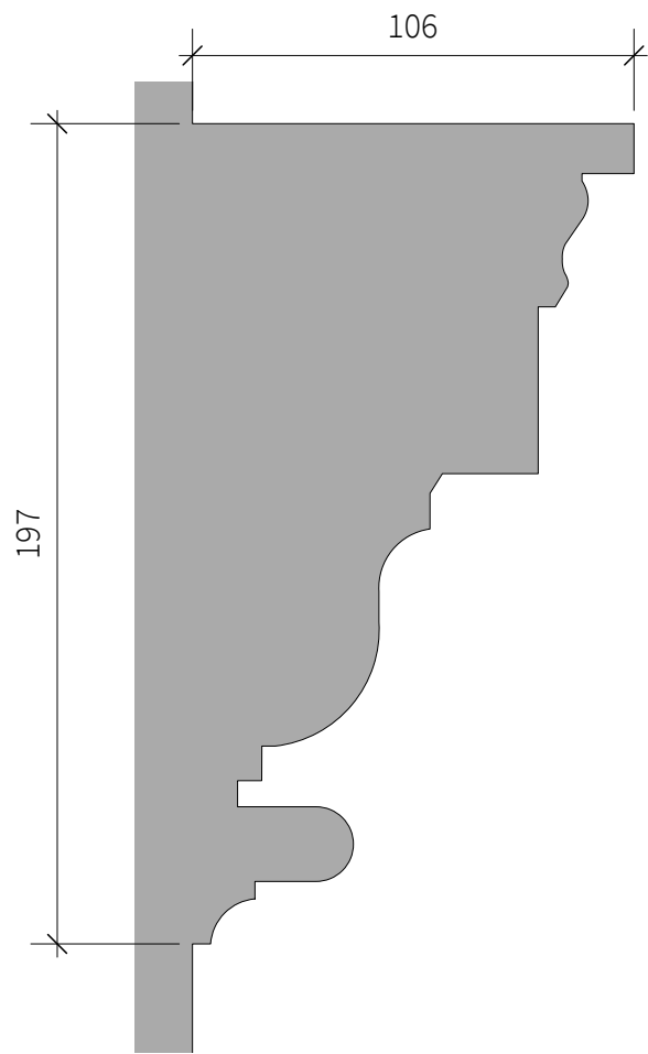
Proposed Capital Details to Columns 1:2
