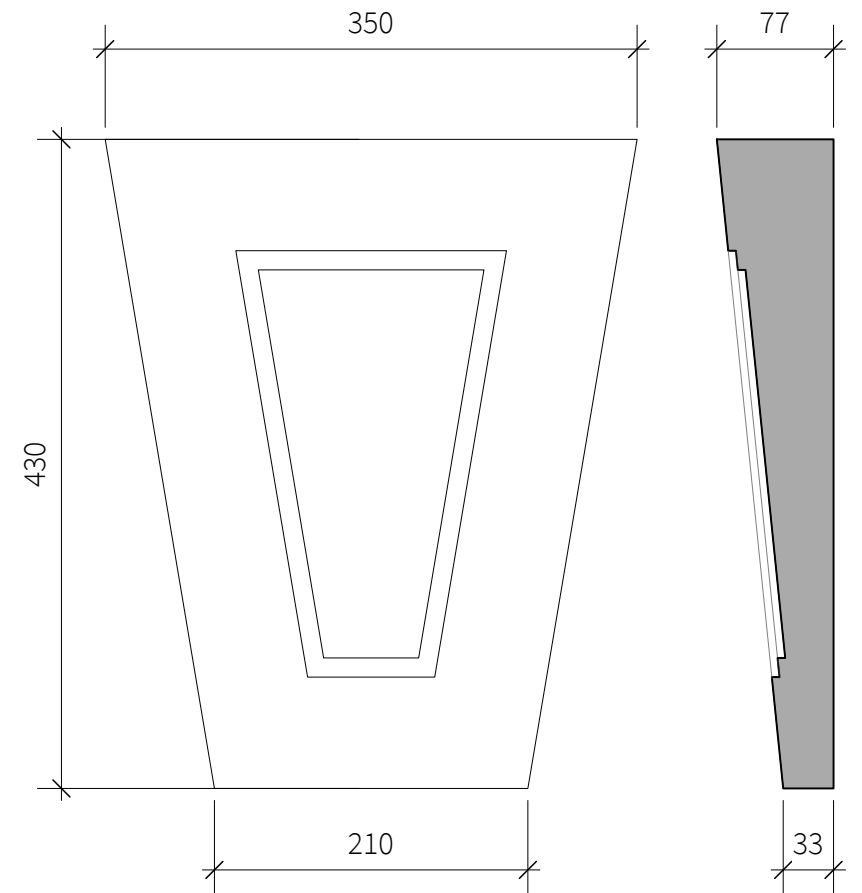
Proposed Keystone 1:5
