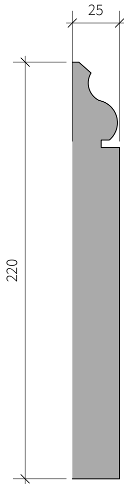
Proposed Skirting and Plinth Details 1:2
