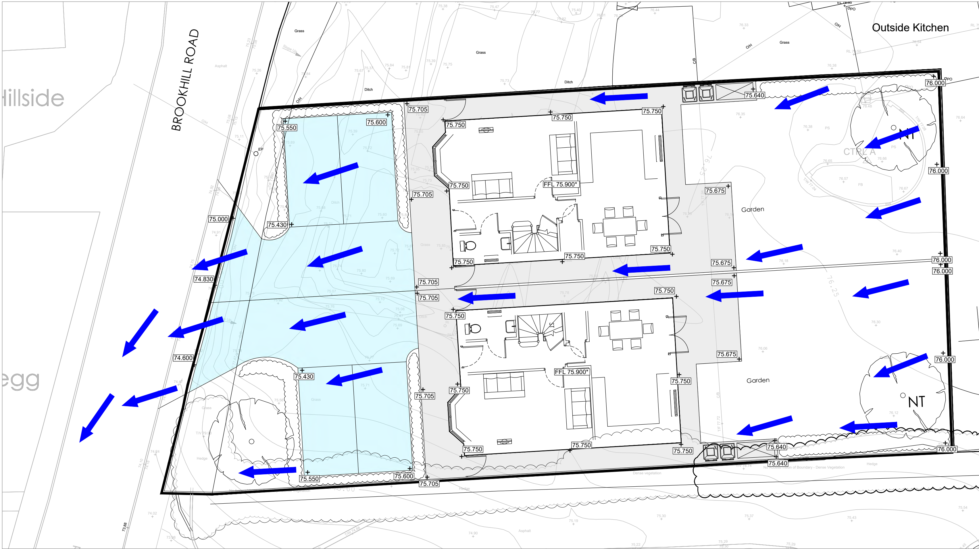
EXCEEDANCE FLOW ROUTES PLAN (scale 1:100)
