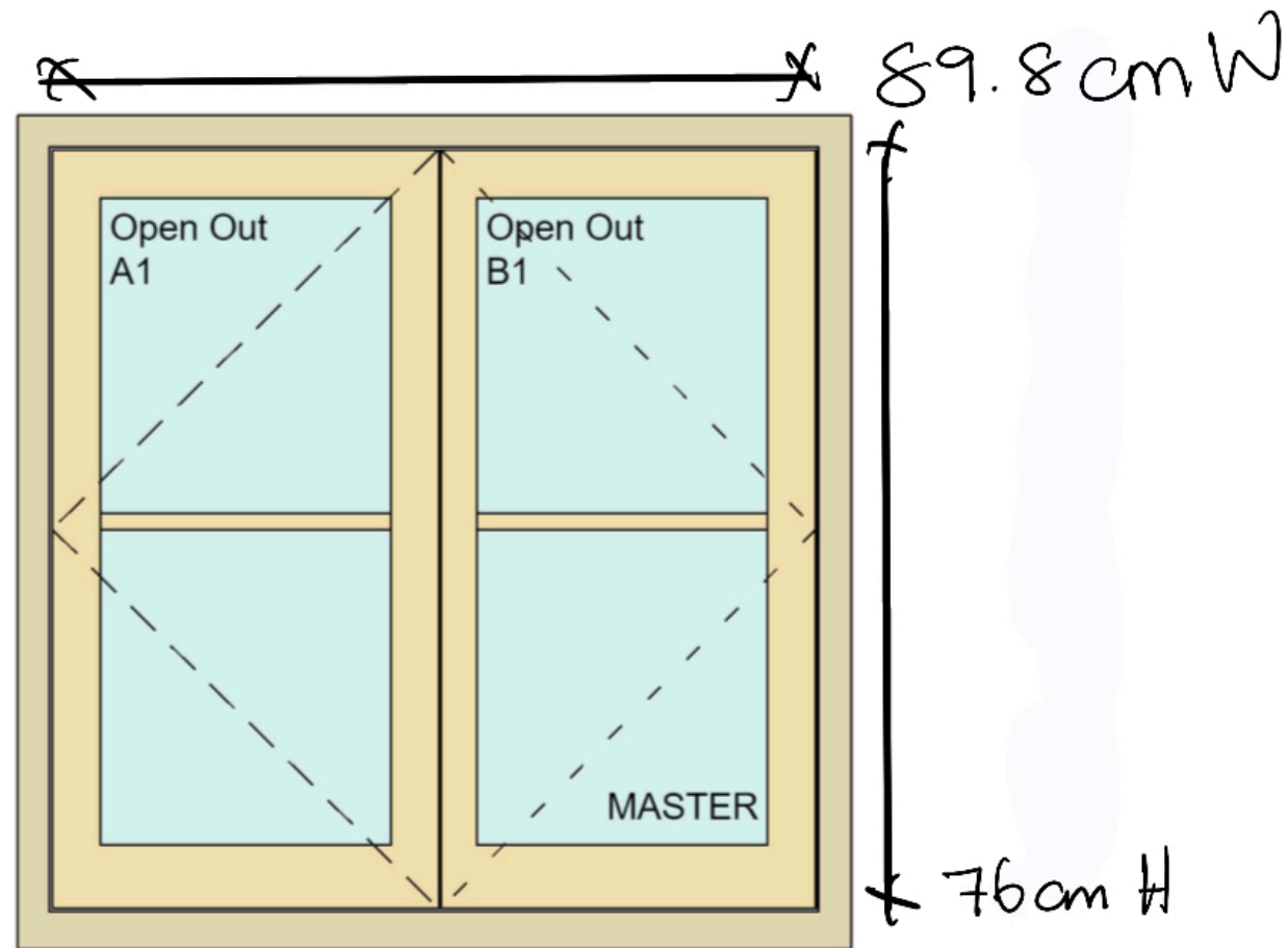
ITEM 7 - First Floor Front Elevation Bedroom 3
