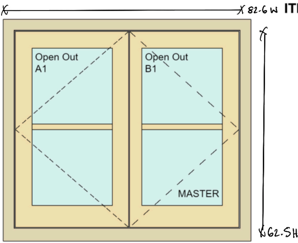
ITEM 12 - Ground Floor Rear Elevation Kitchen M
