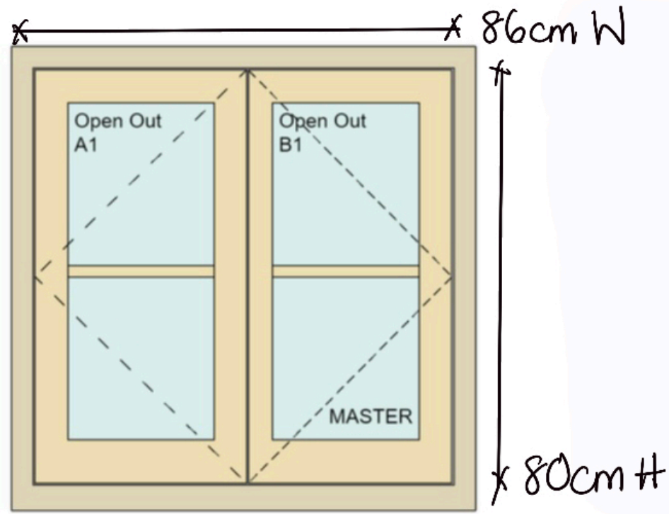
ITEM 1 - Second Floor Rear Elevation Master Bedroom
