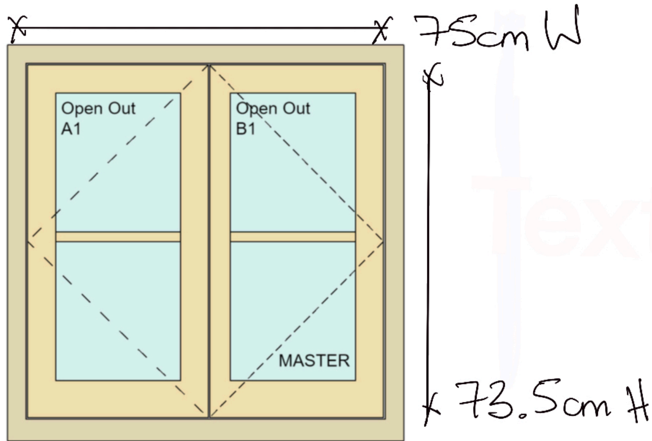
ITEM 3 - Second Floor Rear Elevation En suite
