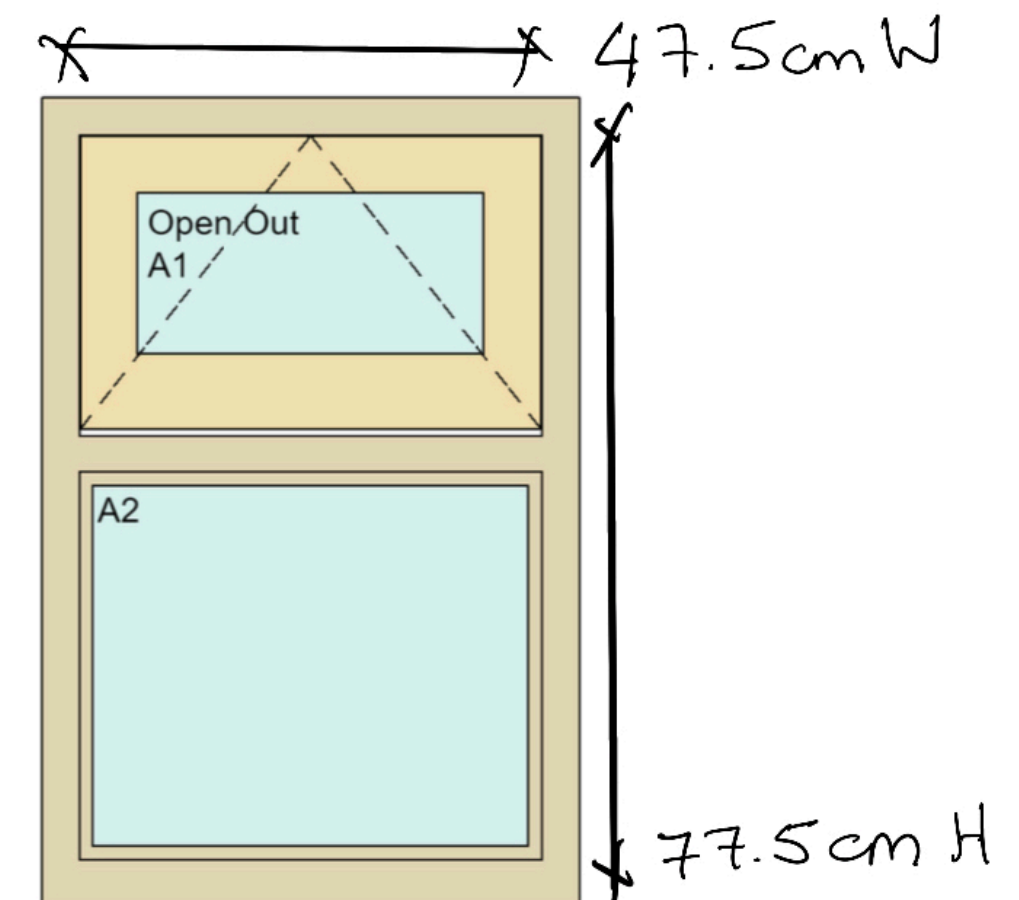
ITEM 8 - First Floor RHS Elevation Stairwell
