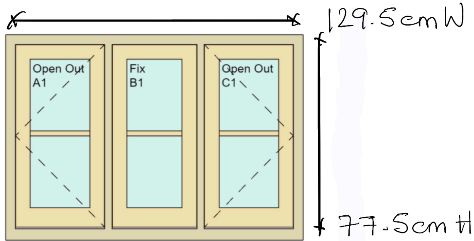
ITEM 5 - First Floor Front Elevation Bedroom 2
