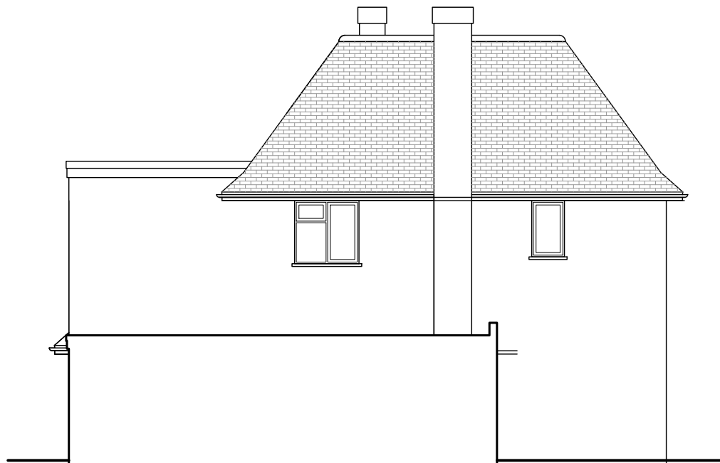
Proposed LHS Elevation Scale 1/100@A3
