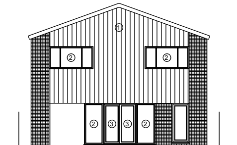
South elevation
