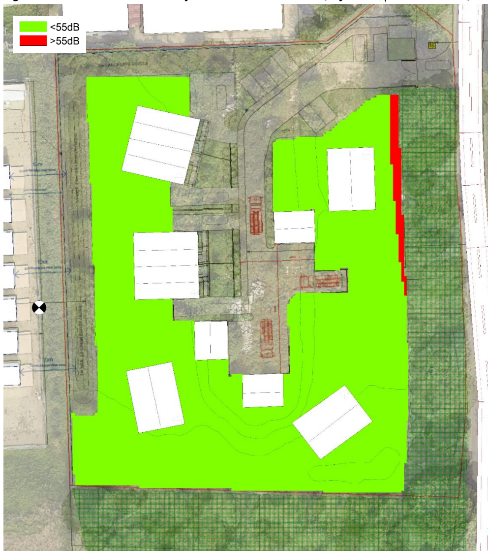
Figure 7.1: Predicted external amenity noise levels across the site (daytime L_{Aeq} free-field levels), dB (1.5m agl)
