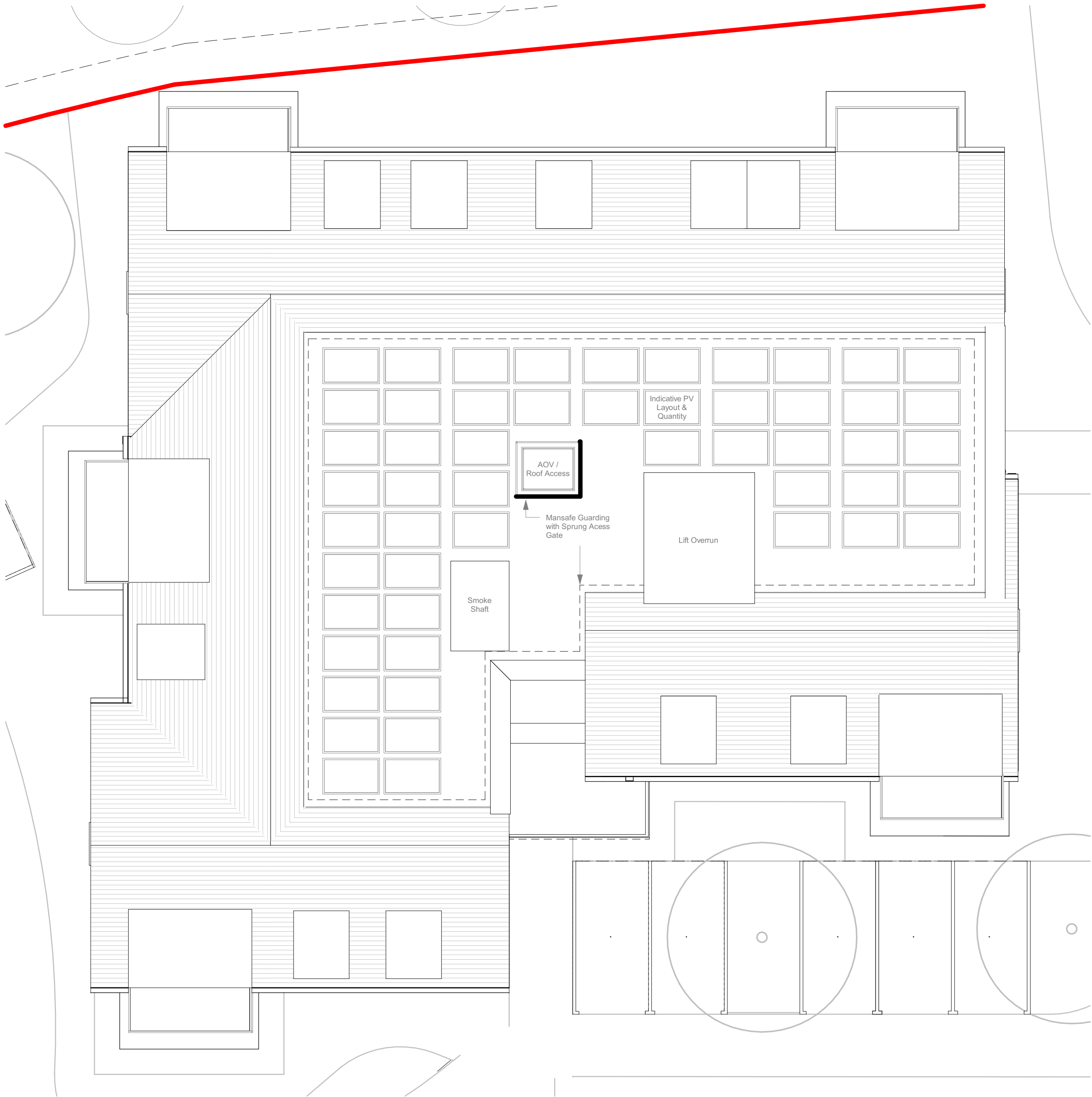
2 Apartment Building A - Roof 1 : 100
