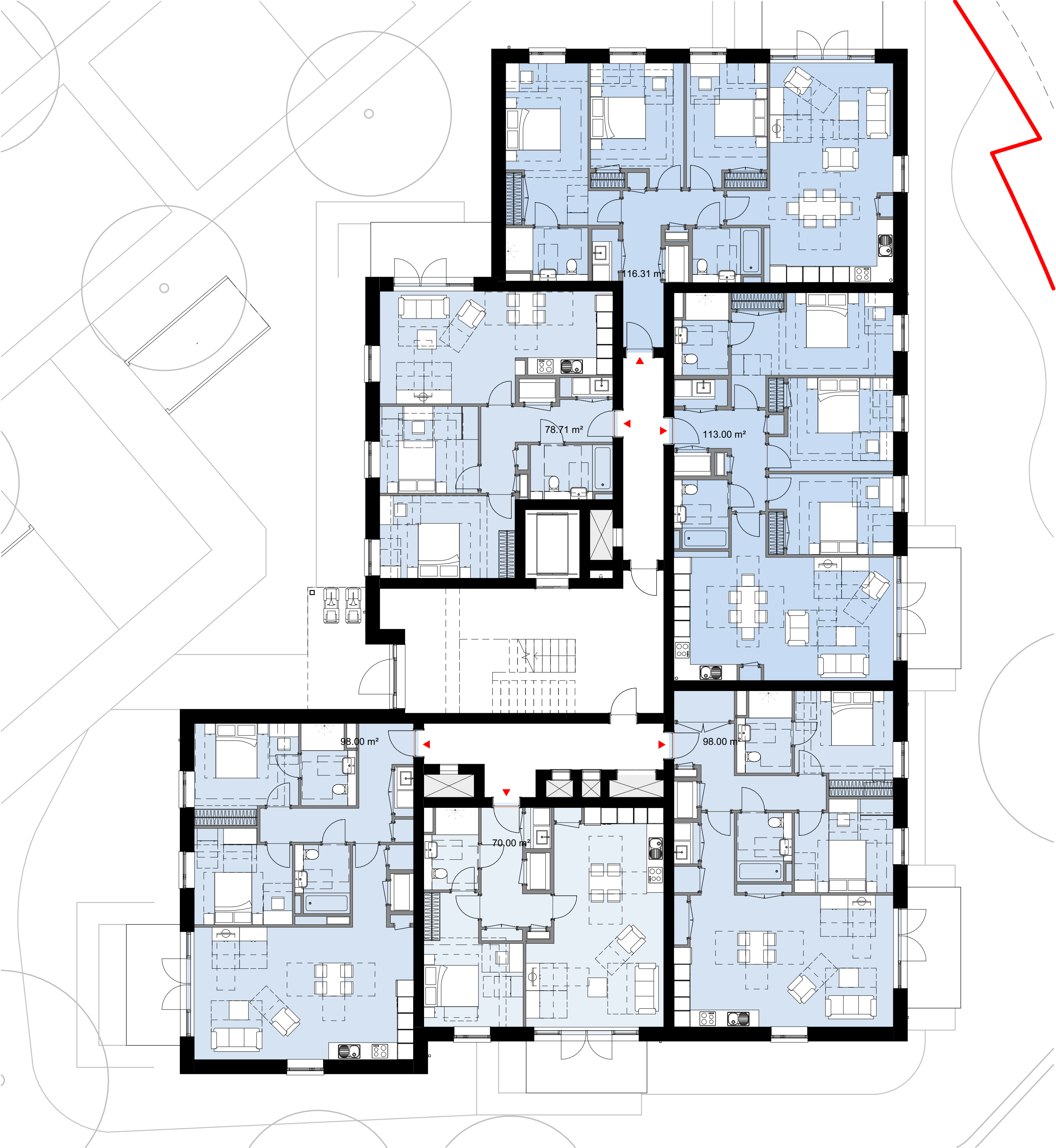
1 Apartment Building B - Level 0 1 : 100
