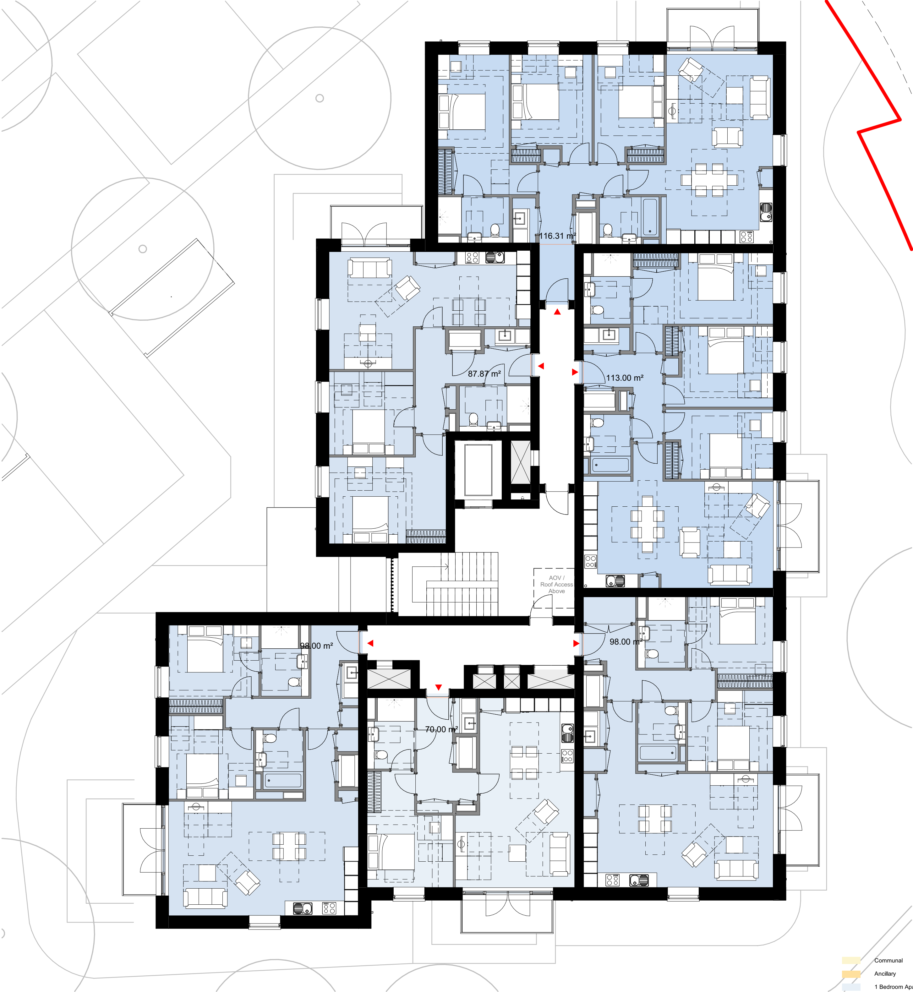
2 Apartment Building B - Level 1 1 : 100
