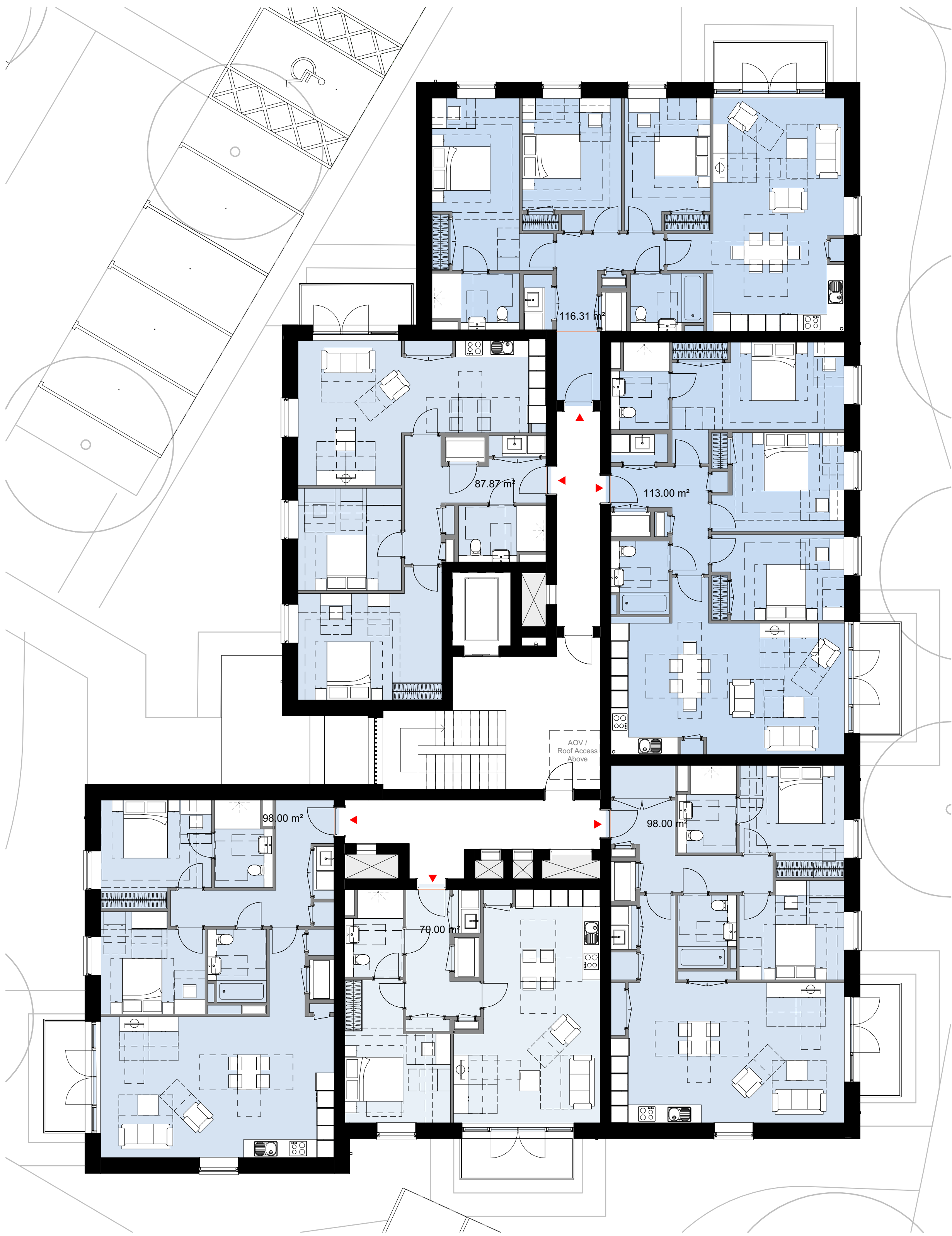
2 Apartment Building C - Level 1 1 : 100
