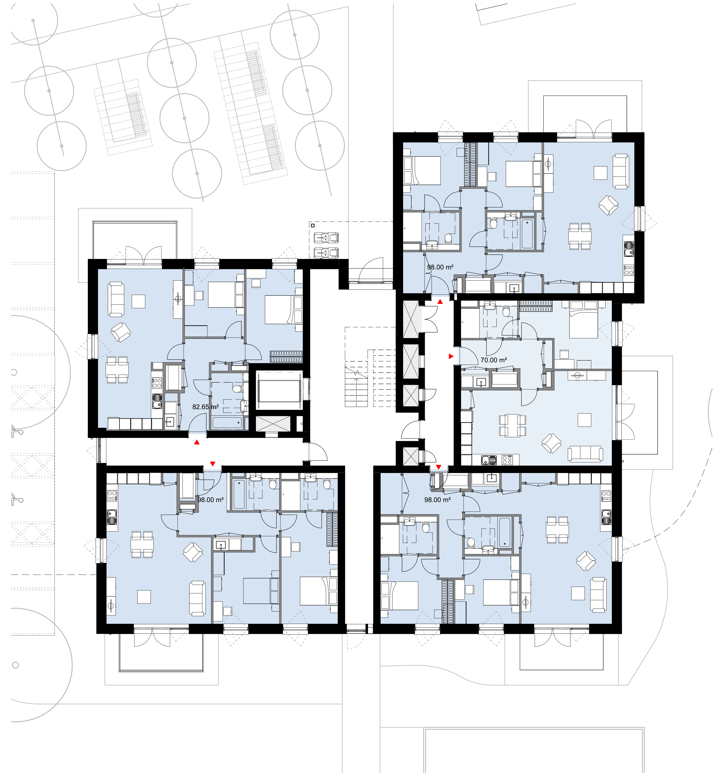
1 Apartment Building E - Level 0 1:100
