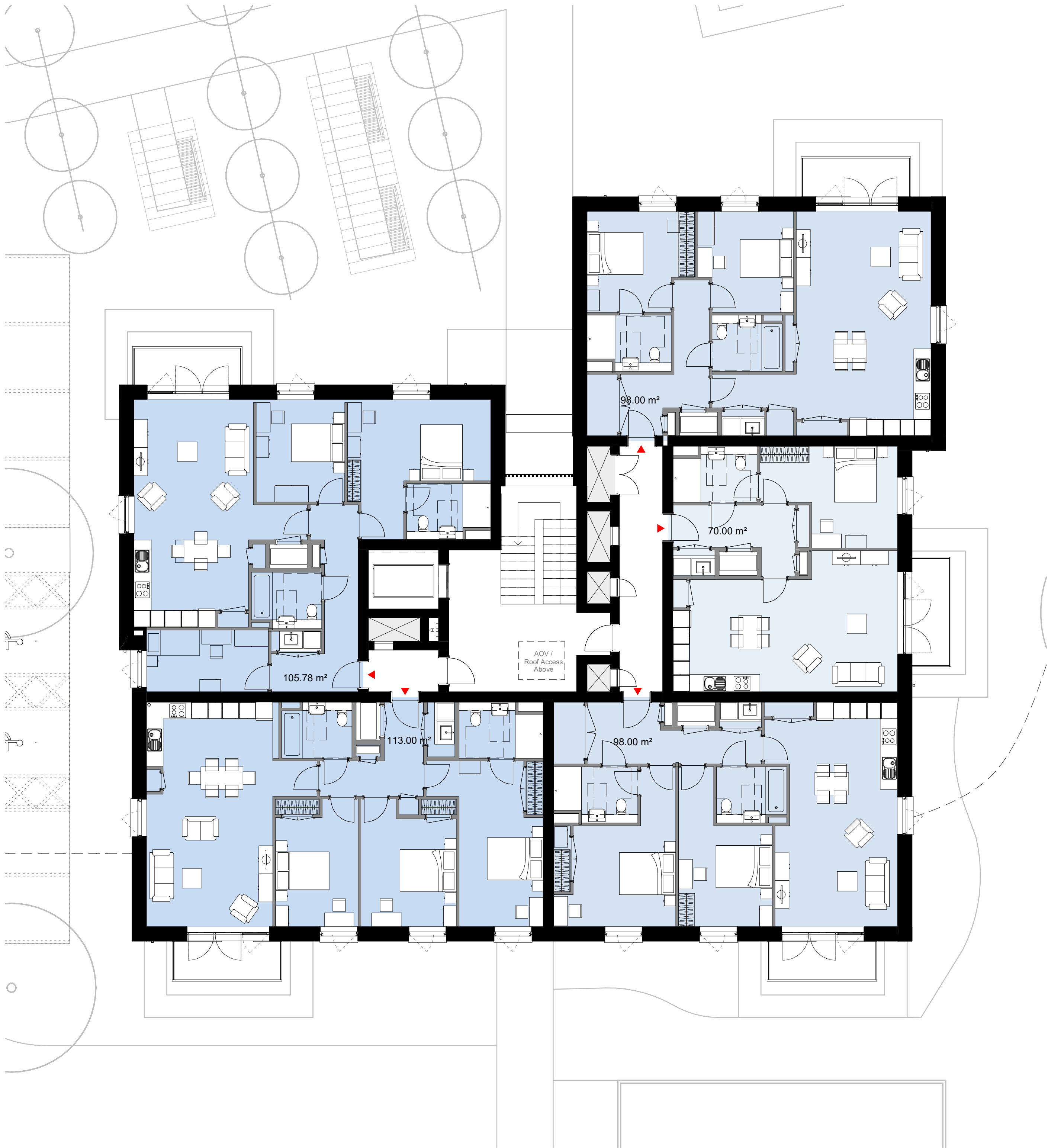
2 Apartment Building E - Level 1 1:100
