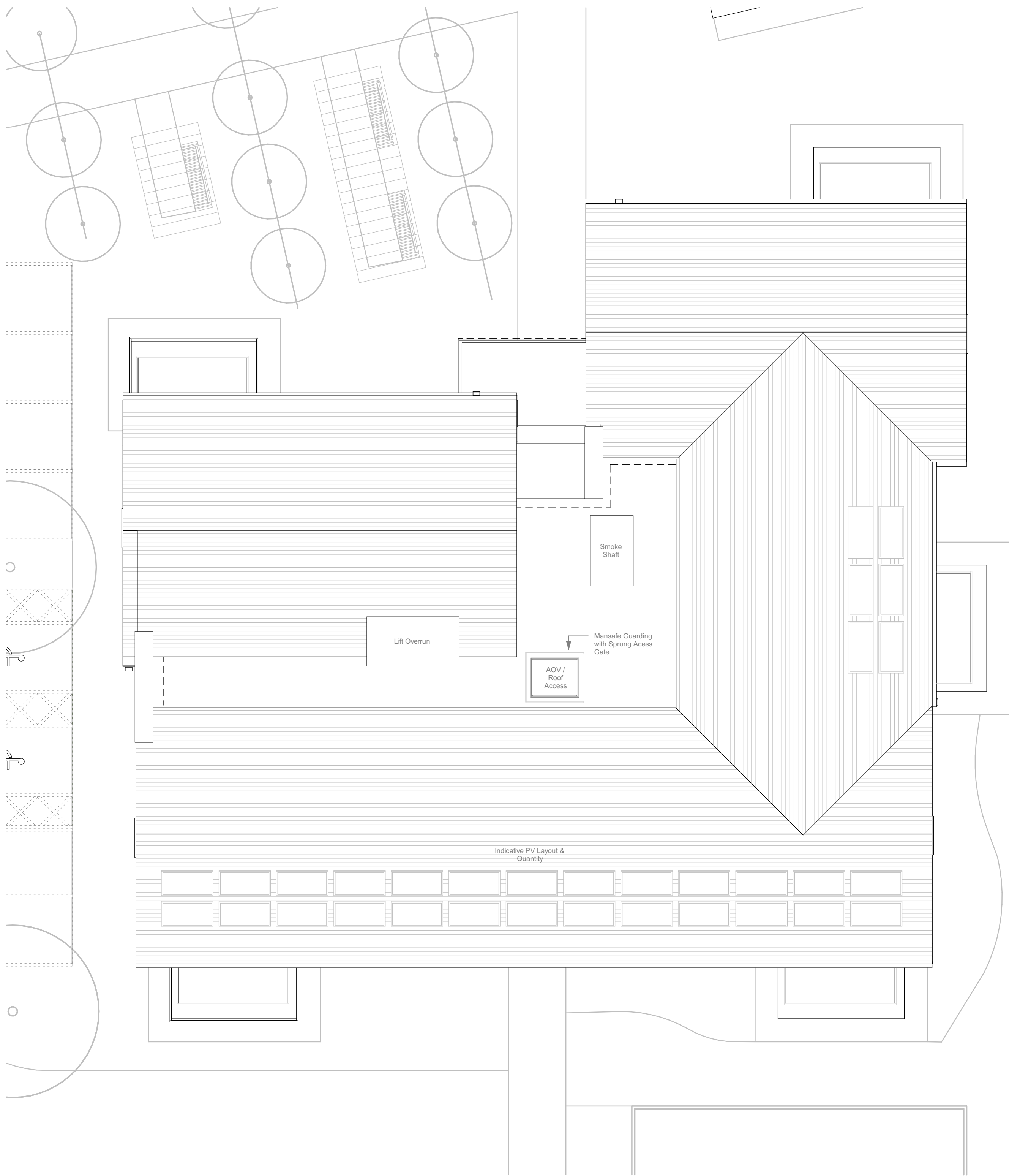
1 Apartment Building E - Roof 1 : 100
