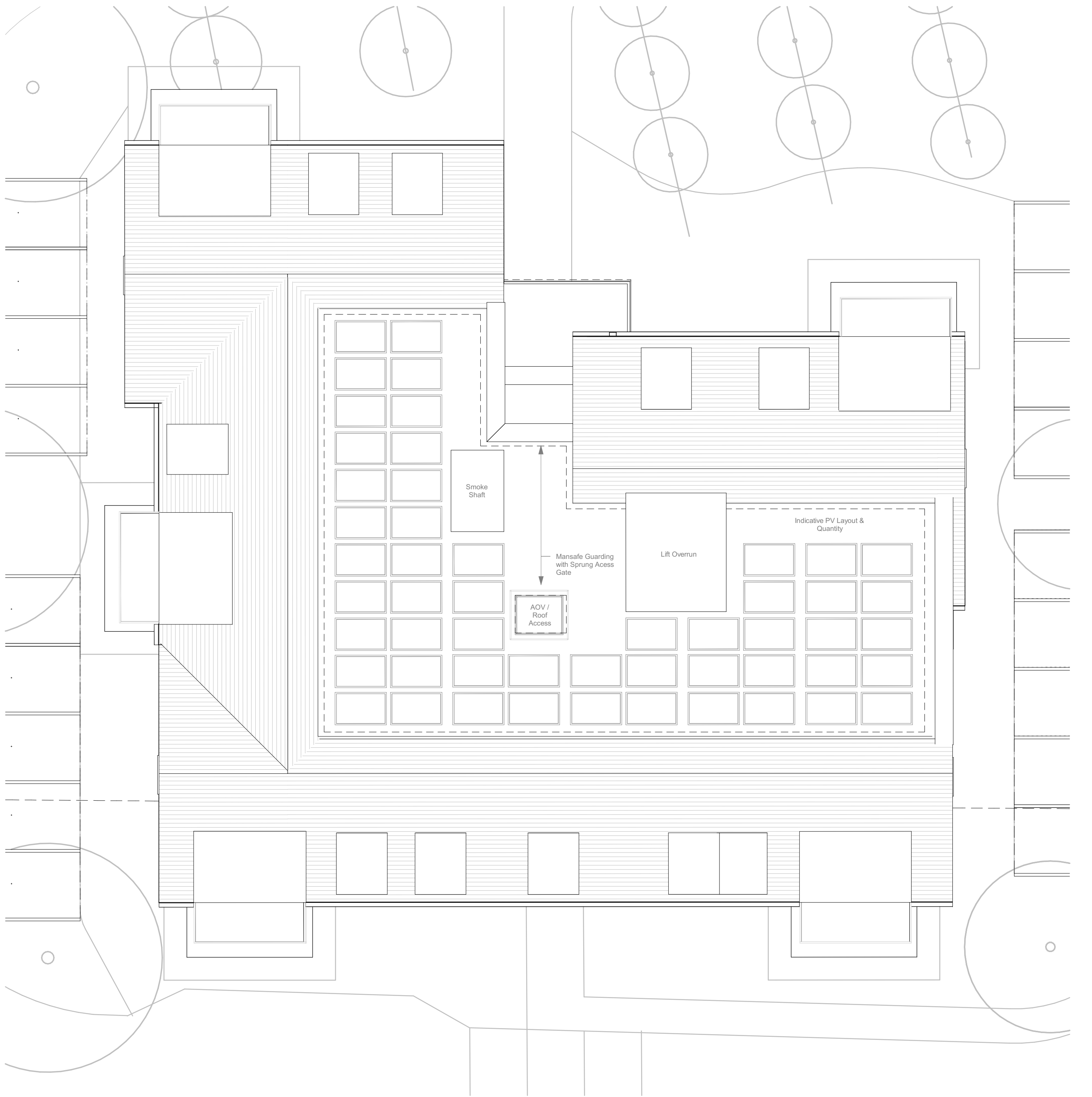
2 Apartment Building G - Roof 1 : 100
