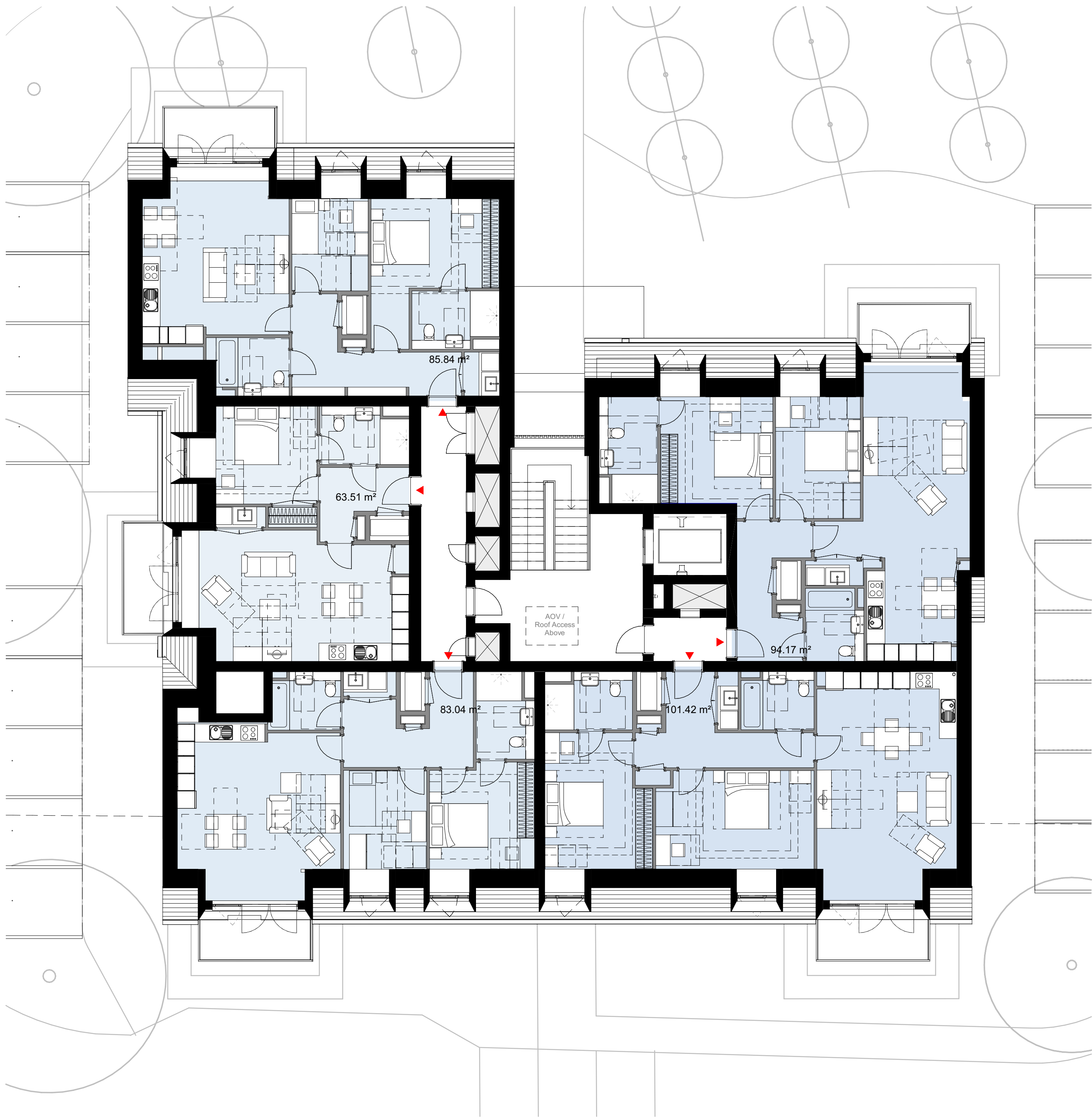
1 Apartment Building G - Level 2 1 : 100
