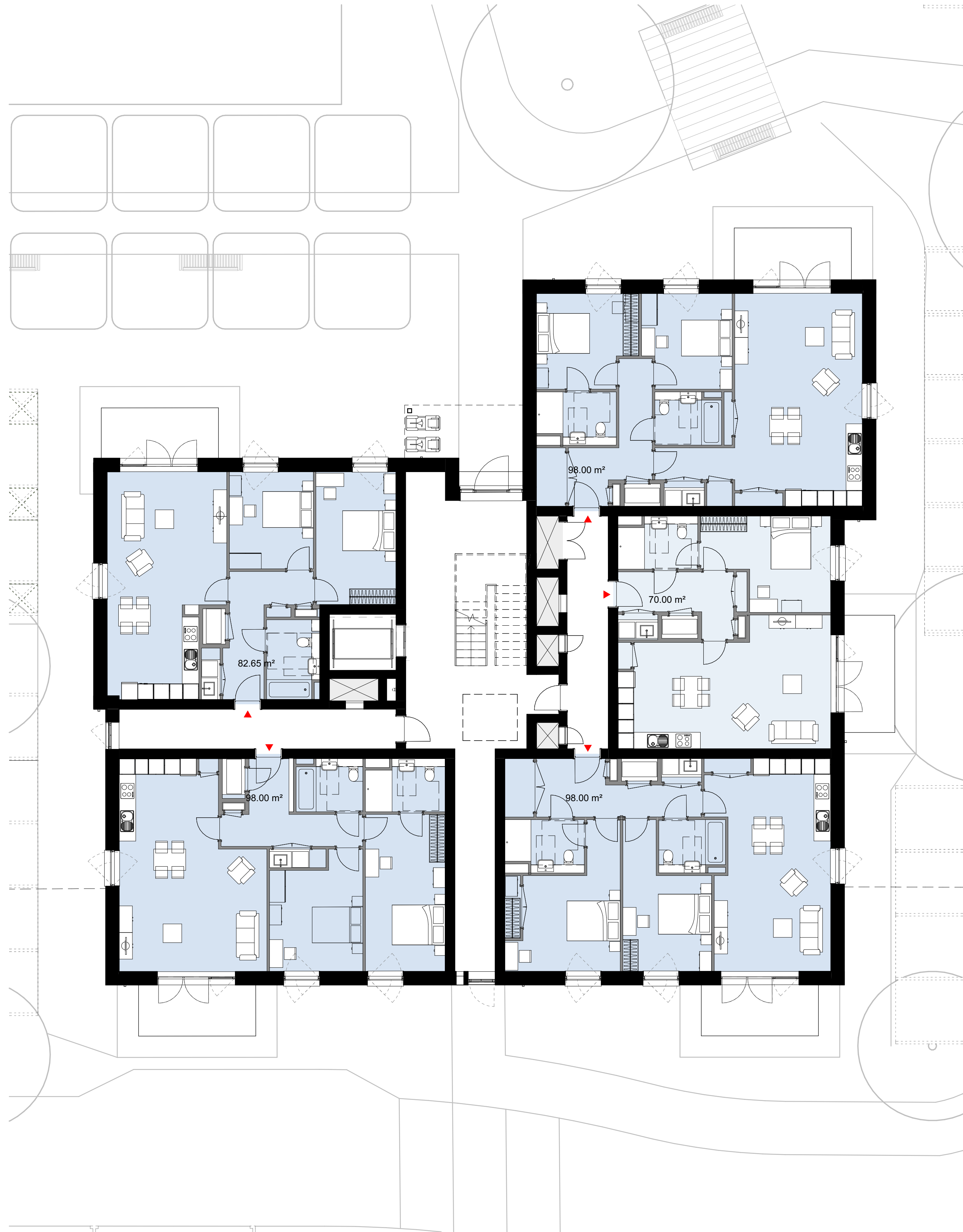
Apartment Building H - Level 0 1 : 100
