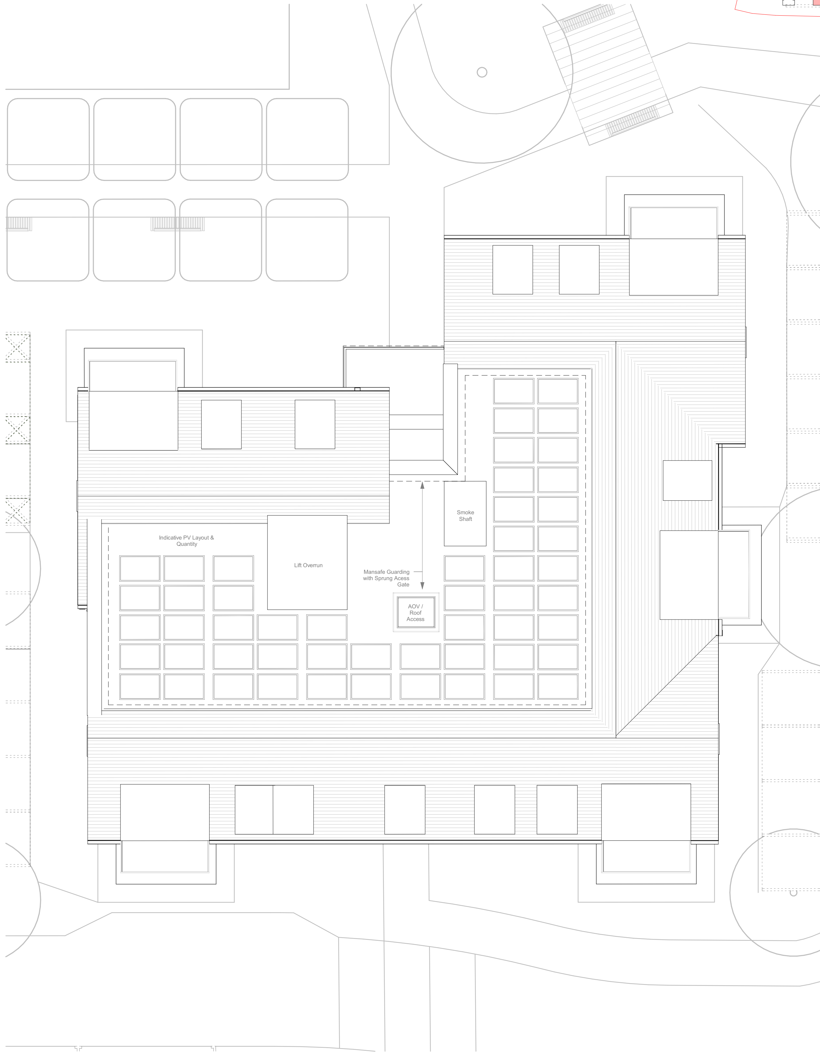
Apartment Building H - Roof 1 : 100
