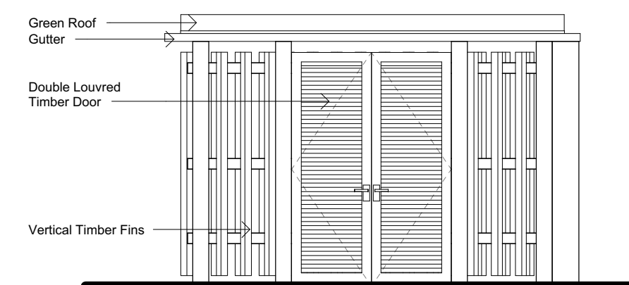
Bin Store D - Elevation 1 - a 1 : 50
