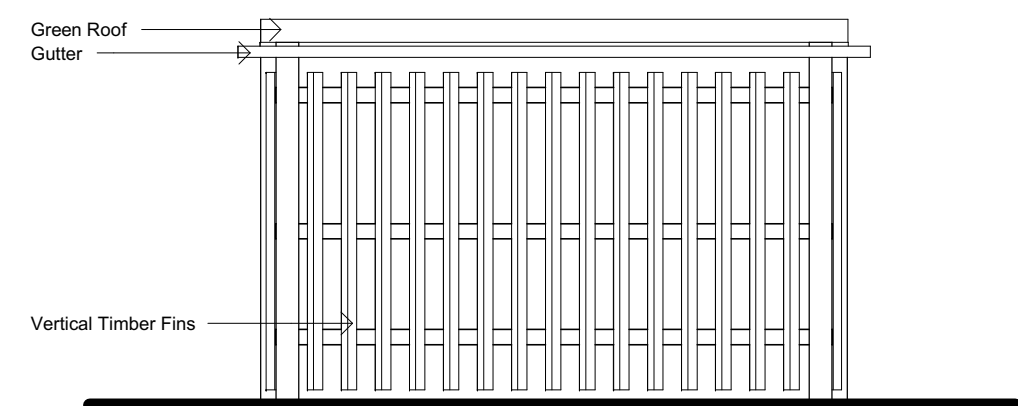
Bin Store A - Elevation 2 - a 1 : 50
