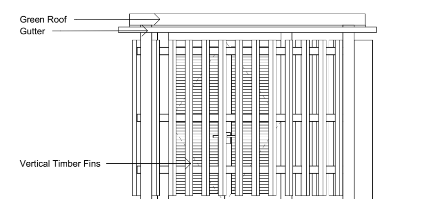
Bin Store C - Elevation 1 - a 1 : 50
