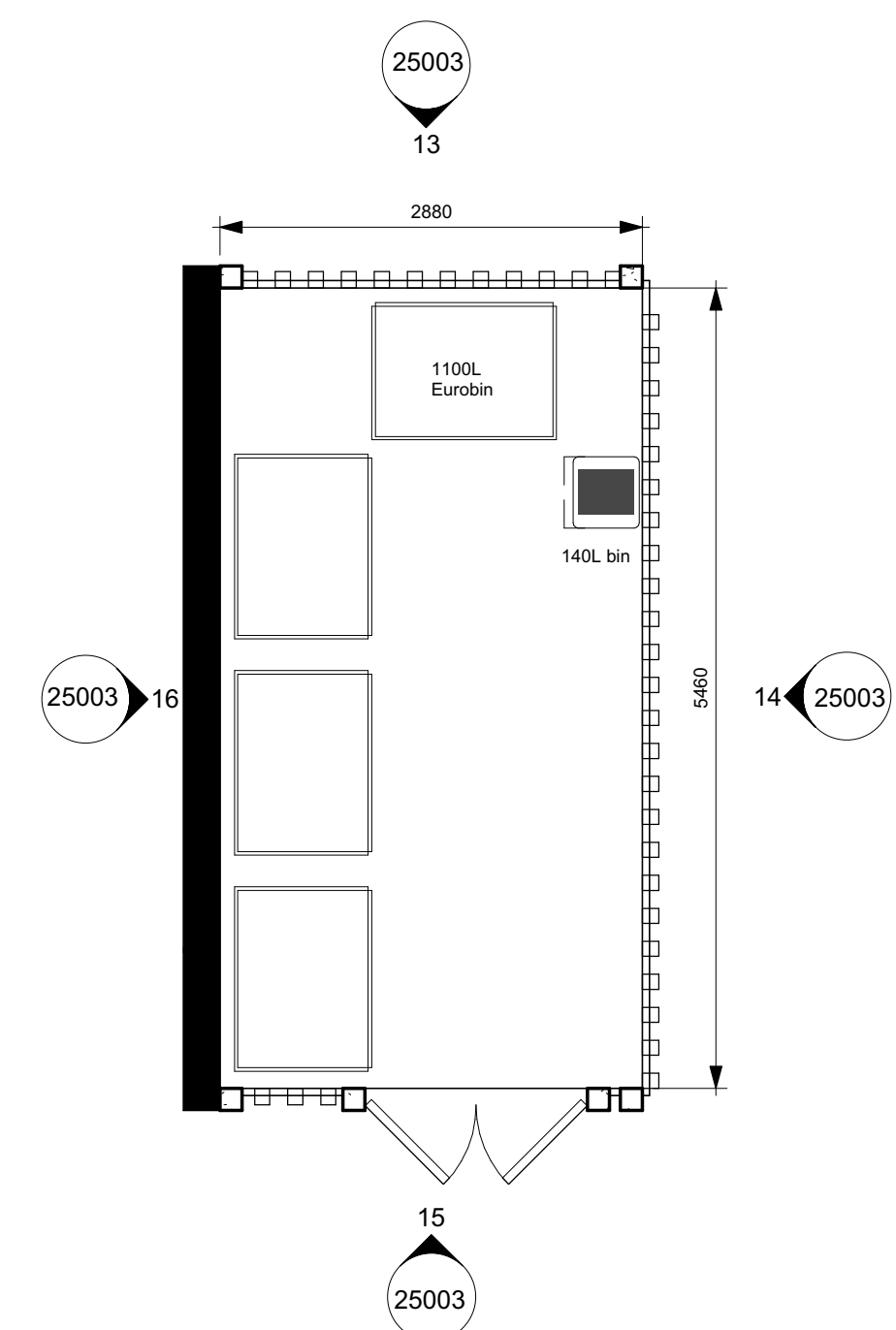
3 | Bin Store C - Level 0 1 : 50
