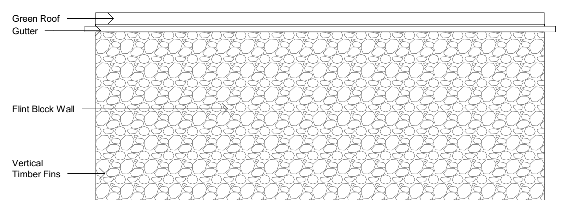
Bin Store D - Elevation 2 - a 1 : 50
