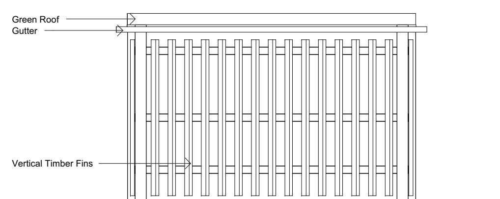
Bin Store A - Elevation 4 - a 1 : 50
