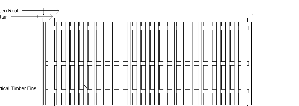
Bin Store B - Elevation 2 - a 1 : 50
