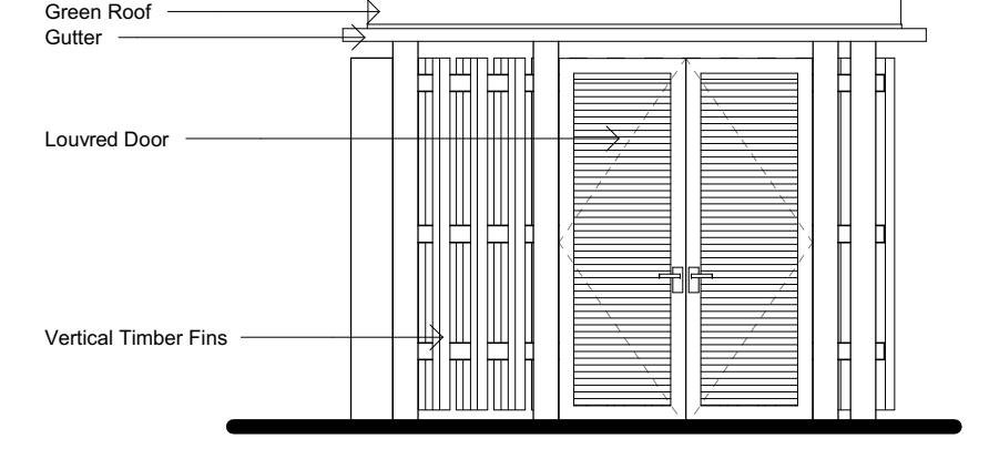
Bin Store C - Elevation 3 - a 1 : 50
