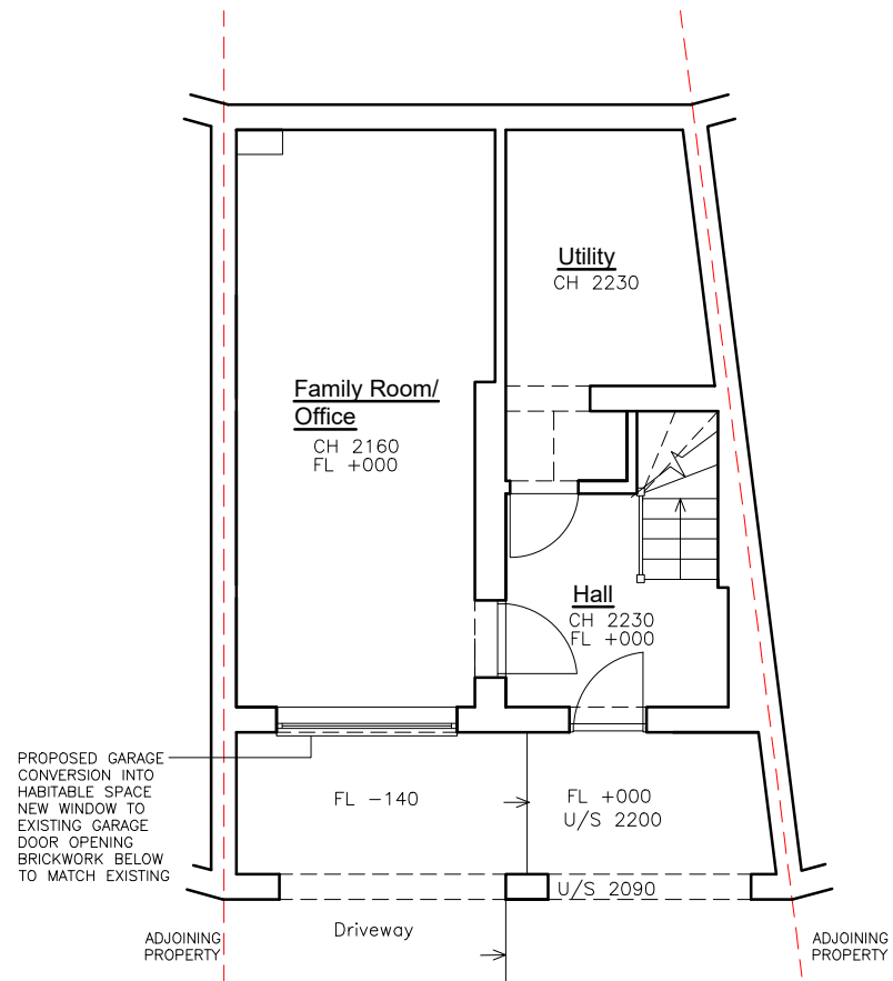
Proposed Lower Ground Floor Plan
