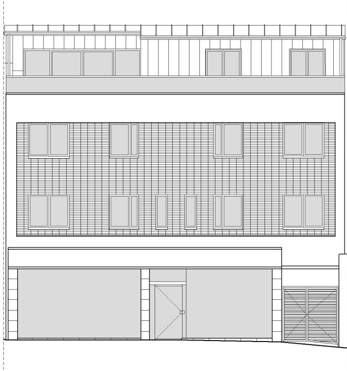
Existing Elevation
