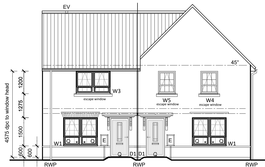
FRONT ELEVATION
