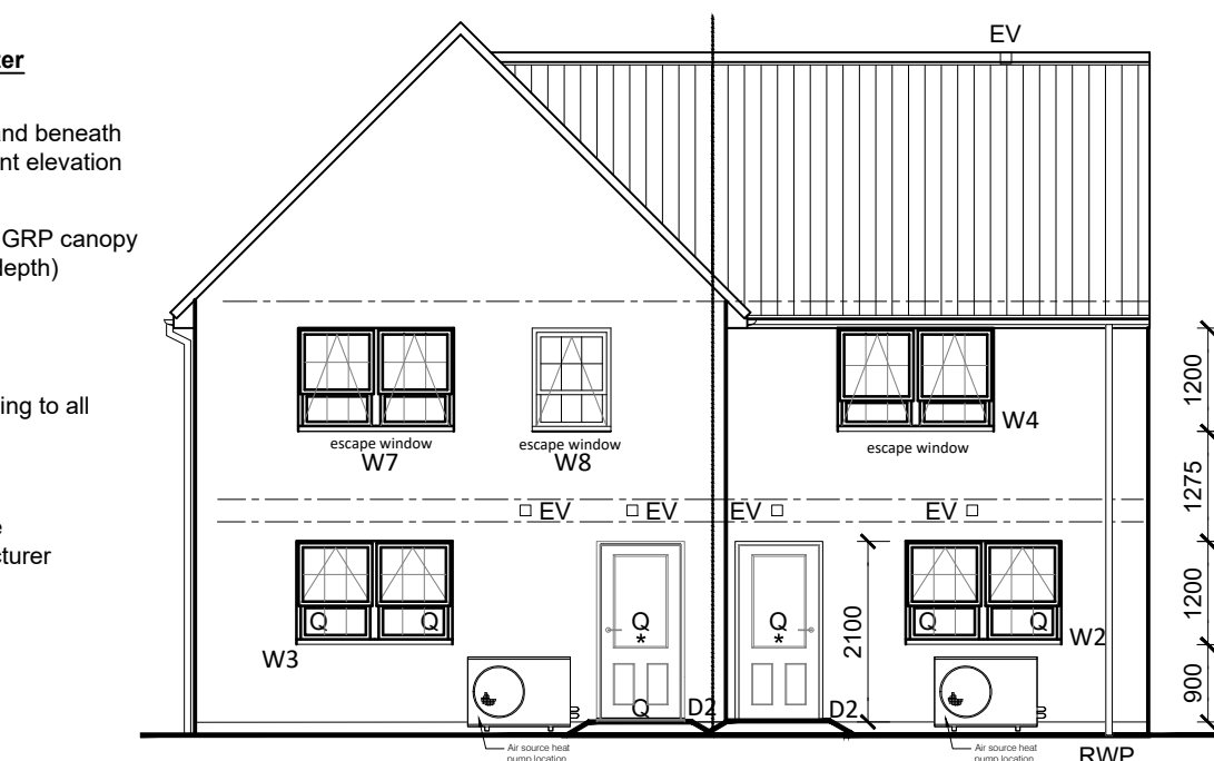
REAR ELEVATION
