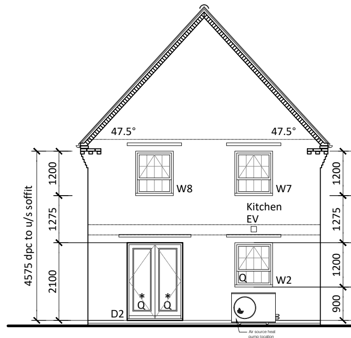
REAR ELEVATION
