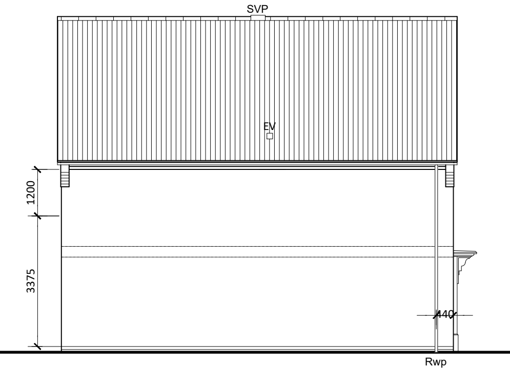
SIDE ELEVATION
