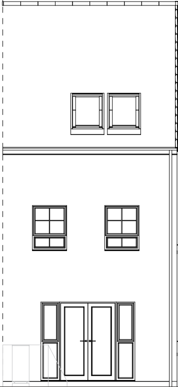
Rear Elevation
