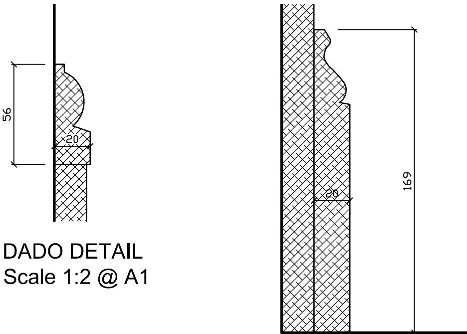
SKIRTING DETAIL Scale 1:2 @ A1
