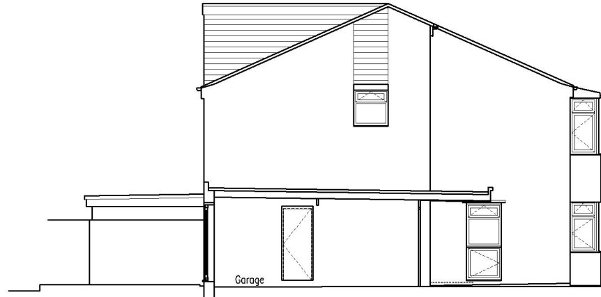
SIDE (SOUTH) ELEVATION SECTION-C
