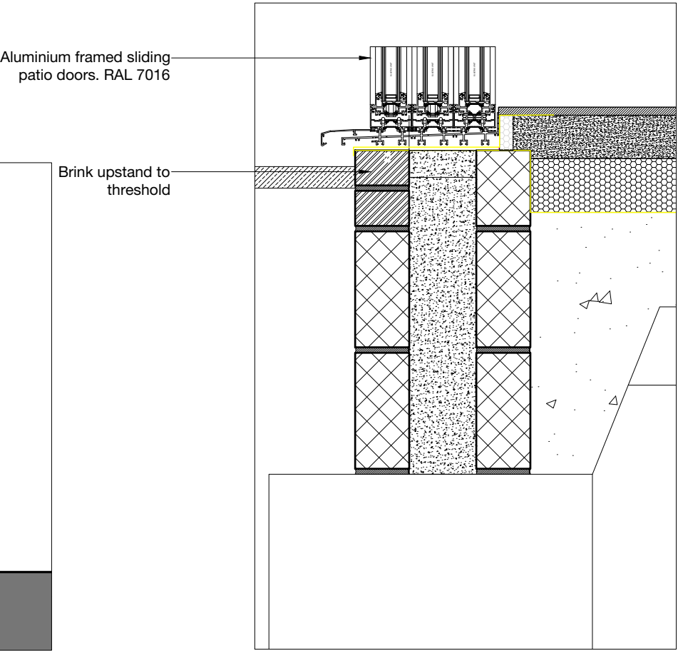
Detailed Section - 1:10
